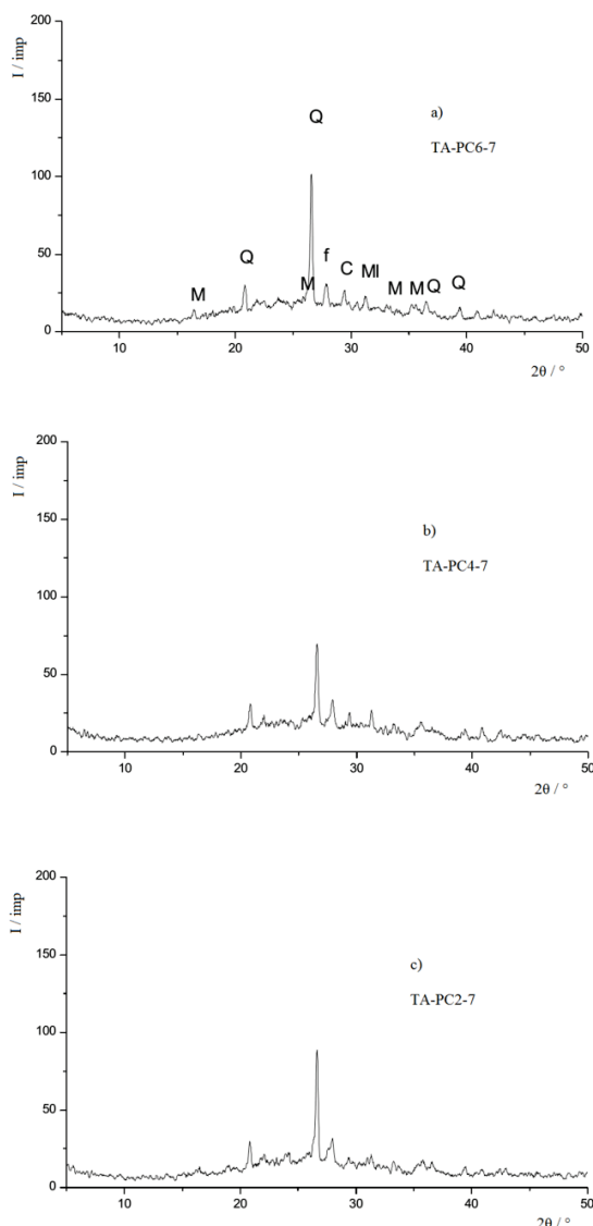
Figure 3 The X-ray diagram of the sample exposed to 7 days in a humid environment with the addition of cement binder: a) 6%, b) 4%, c) 2%
