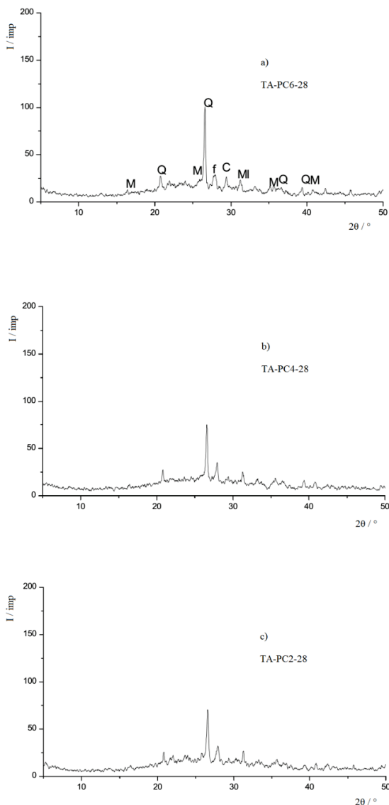
Figure 6 The X-ray diagram of the sample, exposed for 28 days in a humid environment with the addition of cement binder: a) 6 %, b) 4 %, c) 2 %
