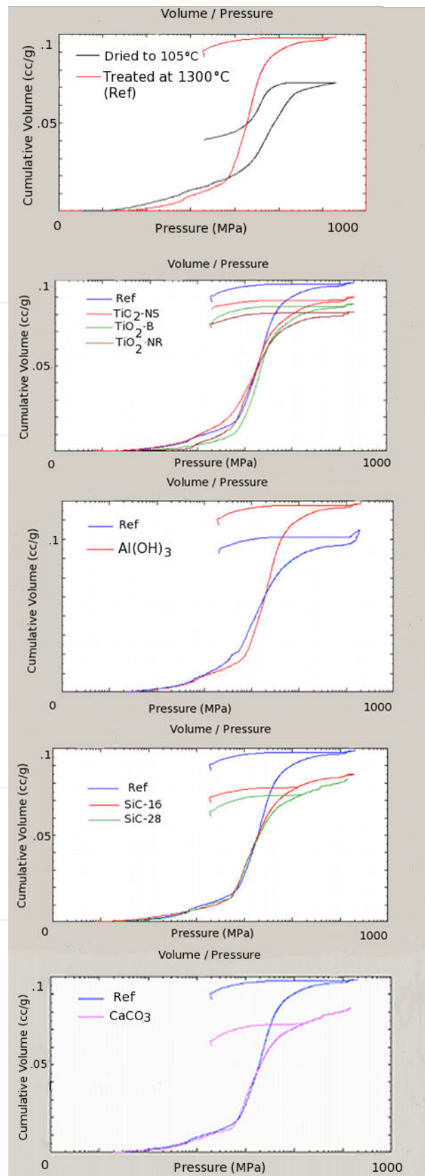
Figure 5. Cumulative infiltration volume versus applied pressure (2 % wt. thermally treated samples). In the figure, Ref stands for the commercial brick without nanocrystals and thermally treated at 1300 °C.
