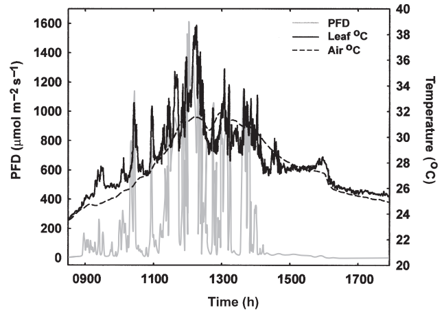
Figure 1. Representative traces over the diurnal period of: leaf temperature (black line) of a S. leprosula seedling in a tropical rainforest understorey, PFD incident on the leaf (grey line) and air temperature (dashed line).
