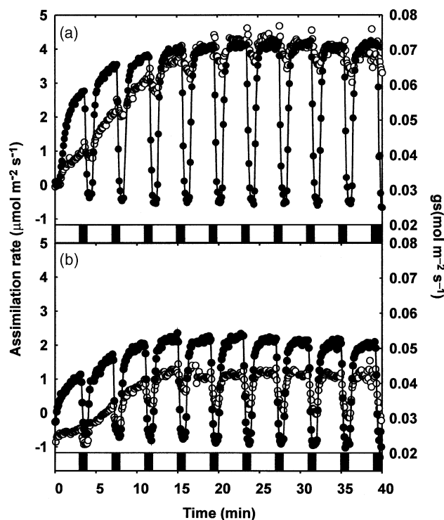
Figure 3. Representative time courses of net photosynthetic rates (closed circles, solid lines) and stomatal conductance (open circles) of S. leprolosula measured at (a) 28 and (b) 38 °C, during a simulated sequence of sunflecks. Flecks are of 3 min duration (white bands) separated by 1 min shade periods (dark bands).
