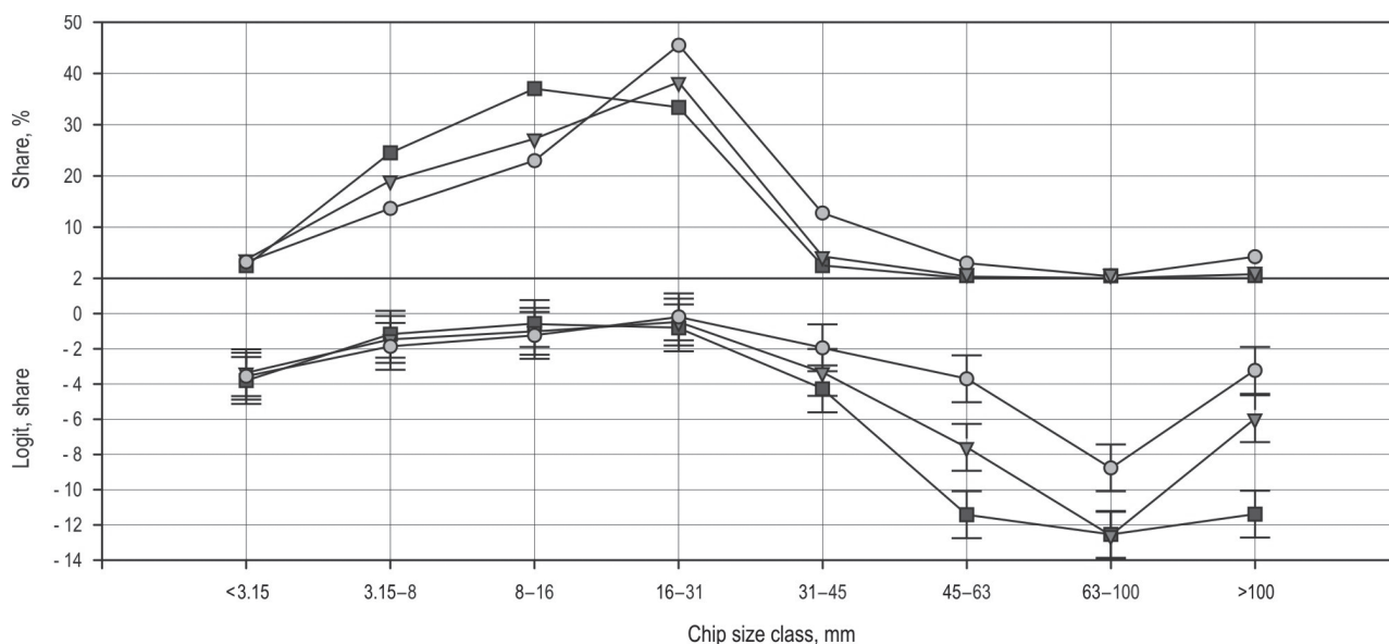
Fig. 2 Chip size distribution as an effect of sieve size, upper part of the figure actual shares in per cent per class, lower part of the figure logit transformed data with 95 % confidence intervals. Coarse sieve denoted by black dots, medium sieve by triangles and fine sieve by squares
