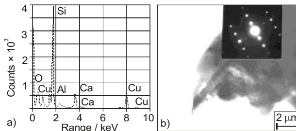
Figure 11. X-ray spectrum (a) and micrograph (b) of the nanocrystalline precipitate of solecism Slika 11. a) EDX, b) mikrograf nekristaličnog precipitata silicija
