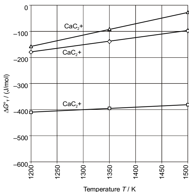
Figure 2. The thermodynamical potential of reaction \Delta G^\circ_T of calcium carbide ( \text{CaC}_2 ) with the oxides \text{Al}_2\text{O}_3 , \text{B}_2\text{O}_3 , \text{Na}_2\text{O}
