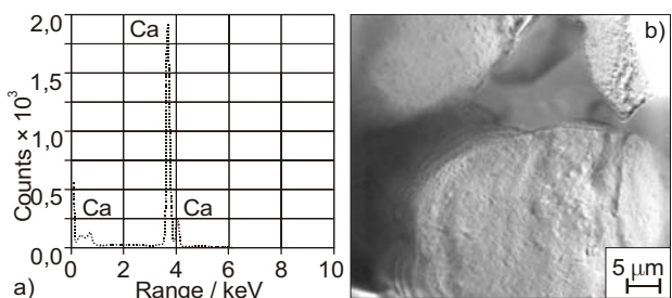
Figure 9. a) X-ray spectrum, b) Transmission electron micrograph of noncrystalline Ca Slika 9. a) EDX, b) TEM nekristaličnog Ca
