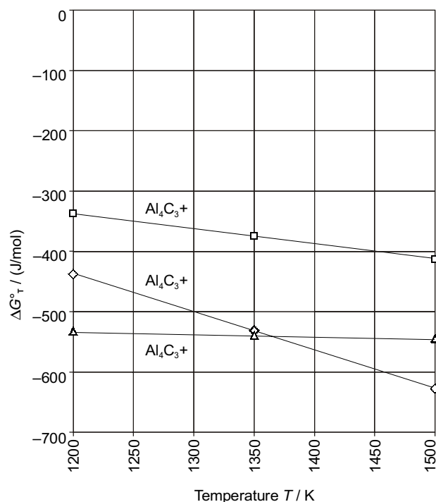
Figure 3. The thermodynamical potential of reaction \Delta G^\circ_T of aluminium carbide ( \text{Al}_4\text{C}_3 ) with the oxides \text{SiO}_2 , \text{B}_2\text{O}_3 , \text{Na}_2\text{O}
