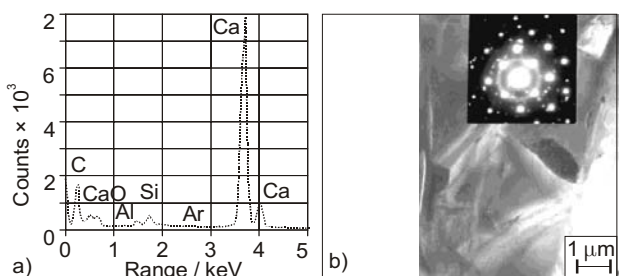
Figure 10. X-ray spectrum (a) and micrograph (b) of the nanocrystalline precipitate of calcium Slika 10. a) EDX, b) mikrograf nekristaličnog precipitata kalcija
