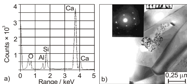
Figure 12. X-ray spectrum and micrograph of the complex compounds formation Slika 12. a) EDX, b) mikrograf stvaranja složenih spojeva
