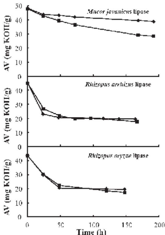
Fig. 5 – Change in acid value as a function of time in the esterification of polyglycerol with polyricinoleic acid performed by free and immobilized lipases, in the atmospheric reactor. Experimental conditions: reaction mixture, molar ratio PR/PG \approx 3; temperature, 40 °C; catalyst ( \blacklozenge ) 0.5 g of free lipase dissolved in 5 ml of distilled water, ( \blacksquare ) 5 g of immobilized derivative and the amount of water soaked into the support (3 ml).
