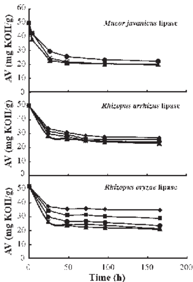
Fig. 3 – Influence of the amount of biocatalyst on the acid value in the esterification of polyglycerol with polyricinoleic acid in the atmospheric reactor using different free lipases. Experimental conditions: reaction mixture, molar ratio PR/PG \approx 3; temperature, 40 °C; enzyme, ( \blacklozenge ) 1.39 mg enzyme/g, ( \blacksquare ) 2.78 mg enzyme/g, ( \bullet ) 6.94 mg enzyme/g, ( \ast ) 13.89 mg enzyme/g, ( \blacktriangle ) 27.28 mg enzyme/g; initial amount of water, 10 \mu L H 2 O/mg enzyme.
