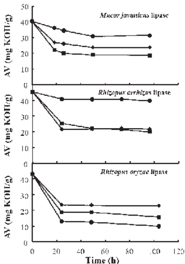
Fig. 4 – Change in acid value as a function of time in the esterification of polyglycerol with polyricinoleic acid in the atmospheric reactor using different free lipases at different temperatures. Experimental conditions: reaction mixture, molar ratio PR/PG \approx 3; enzyme, 0.5 g dissolved in 5 ml of water. ( \blacklozenge ) 40 °C, ( \blacksquare ) 50 °C, ( \bullet ) 60 °C.
