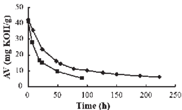
Fig. 8 – Evolution of acid value in the esterification of polyglycerol with polyricinoleic acid in the vacuum reactor, using different enzyme-loading derivatives of Rhizopus oryzae lipase. Experimental conditions: reaction mixture, molar ratio PR/PG \approx 3; temperature, 40 °C; pressure, 160 mmHg; dry air flow, 90 L h -1 ; catalyst, 5 g of the immobilized derivative (♦) 16.36 mg protein/g support, (■) 39.4 mg protein/g support and the amount of water soaked into the support (3 ml).
