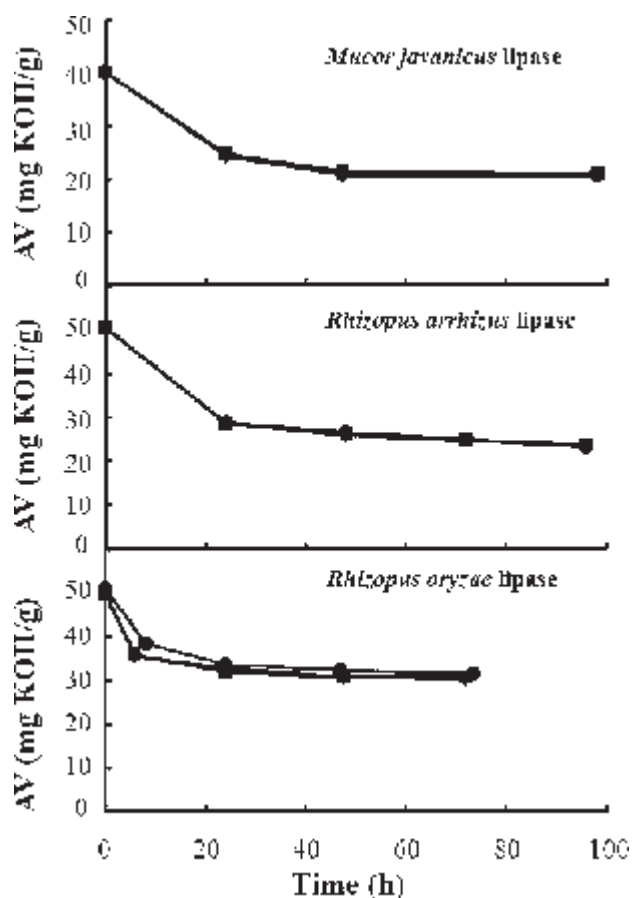
Fig. 2 – Change in acid value as a function of time for the esterification of polyglycerol with polyricinoleic acid in the atmospheric reactor using different free lipases, with different amounts of initial water added. Experimental conditions: reaction mixture, molar ratio PR/PG \approx 3; temperature, 40 °C; enzyme, 0.5 g. ( \blacklozenge ) 1.5 \mu L H 2 O/mg enzyme, ( \blacksquare ) 10 \mu L H 2 O/mg enzyme, ( \bullet ) 20 \mu L H 2 O/mg enzyme.
