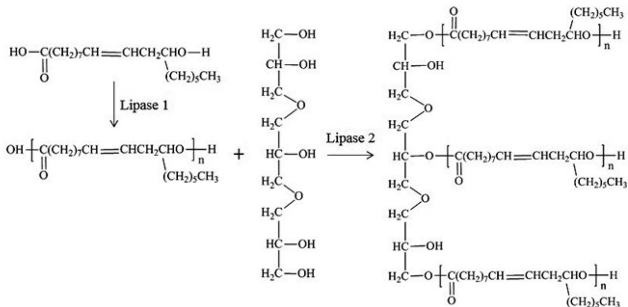
Fig. 1 – Reaction scheme of the synthesis of polyglycerol polyricinoleate (PGPR).
