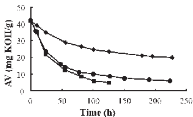
Fig. 7 – Comparison of esterification of polyglycerol with polyricinoleic acid in a vacuum reactor, catalyzed by different immobilized lipases. Experimental conditions: reaction mixture, molar ratio PR/PG \approx 3; temperature, 40 °C; catalyst, 5 g of the immobilized derivative from (◆) Mucor javanicus lipase, (■) Rhizopus arrhizus lipase, (●) Rhizopus oryzae lipase and the amount of water soaked into the support (3 mL); pressure, 160 mmHg; dry air flow, 90 L h -1 .
