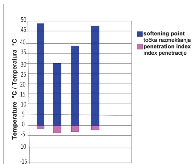
Fig 3. Bar chart showing softening point and penetration index plot of AB, OB, LB and IB.
