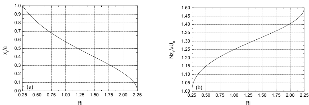
Figure 3. Normalized position of the lowest flow stagnation zone as a function of Ri . (a) horizontal, (b) vertical
