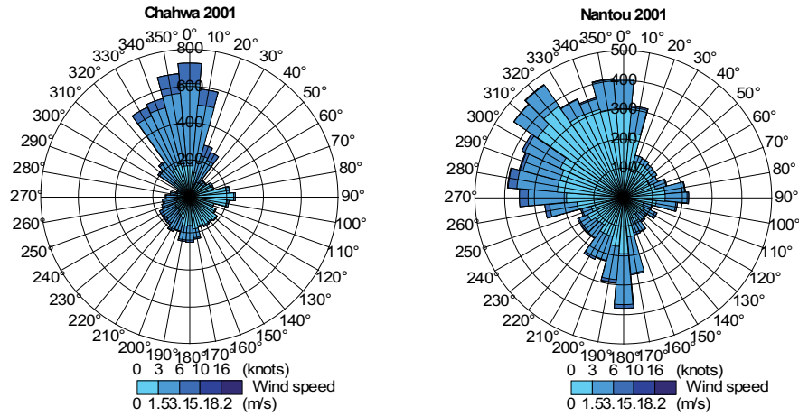
Figure 2. Wind roses of Chahwa and Nantou.
