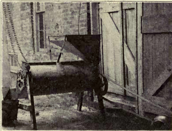
FIG. 27.—MACHINE USED FOR TREATING WHEAT FOR SMUT
