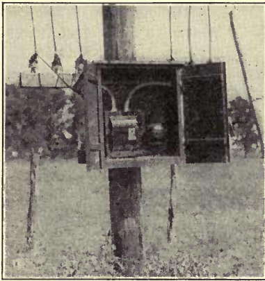
FIG. 3.—TOTALIZING METER AND SWITCHBOX IN BOX ON TRANSFORMER POLE
