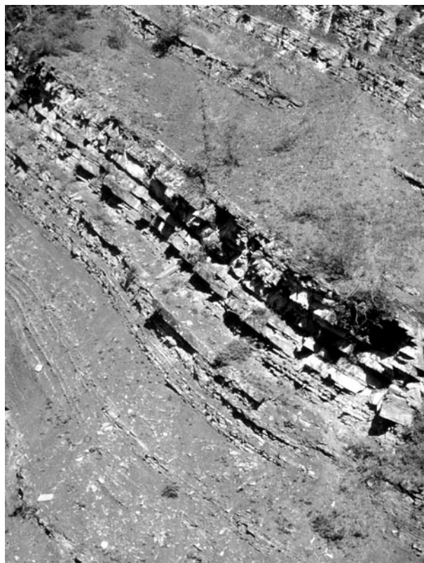
Fig. 6 Three successions of prodelta storm beds grading up into thicker sandstones of the delta front. The main package of sandstone is 4 m thick and is capped by a coal. Flood Creek, Alberta.
