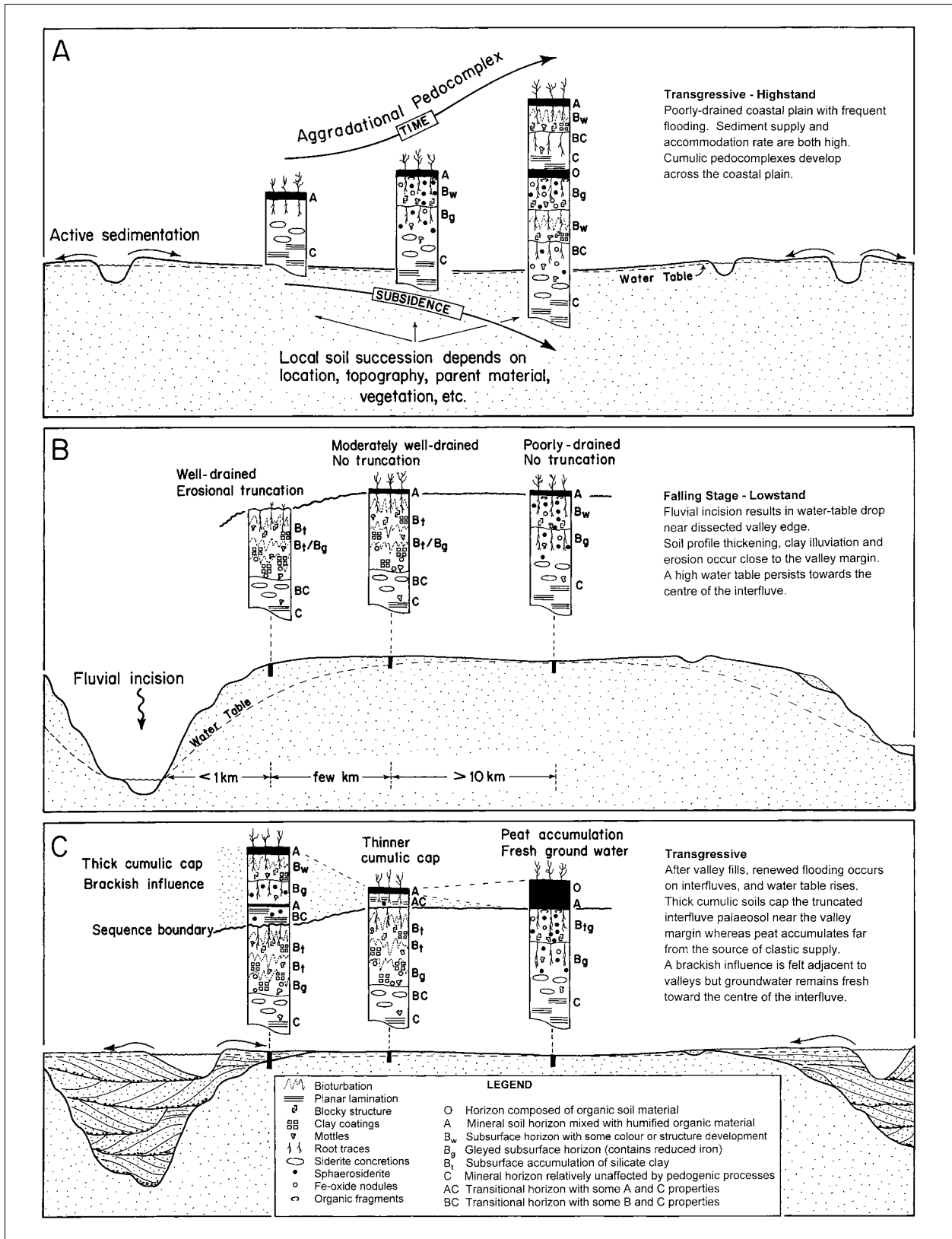
Fig. 22 Diagram summarizing the developmental history of interfluvial palaeosols, and also showing how the history and character of the palaeosol varies with distance from the margins of palaeovalleys. The distance from the valley margin strongly influenced the drainage of the interfluvium, and also controlled the rate of sediment flux once the valley had been filled (from McCARTHY & PLINT, in review).
