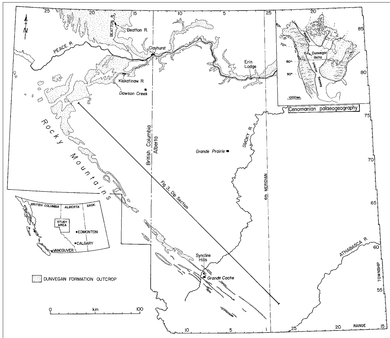
Fig. 1 Inset maps show location of study area in western Canada, and Cenomanian palaeogeography of the Dunvegan Formation within the Western Interior Seaway. The line of section shows the location of the dip section shown schematically in Fig. 3, and drawn to scale in Fig. 23 (from PLINT & WADSWORTH, in review).
