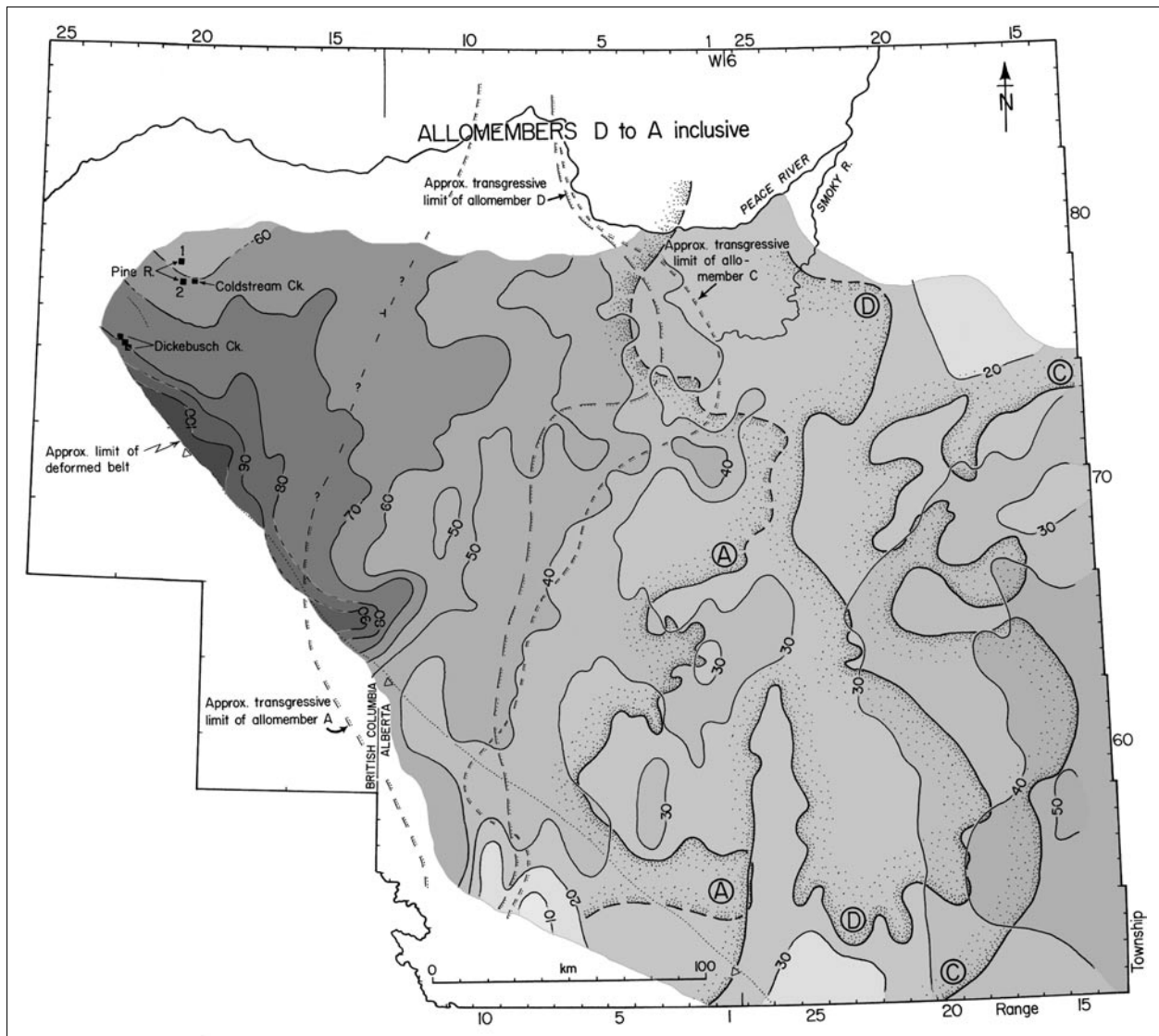
Fig. 16 Composite map showing the maximum progradational shorelines of Dunvegan allomembers D, C and A, and also isopachs for the entire D-A interval. Note the prominent depocentre along the western margin of the study area, and progressive rotation of isopach lines from N-S to NW-SE (from LUMSDON & PLINT, 2003).
