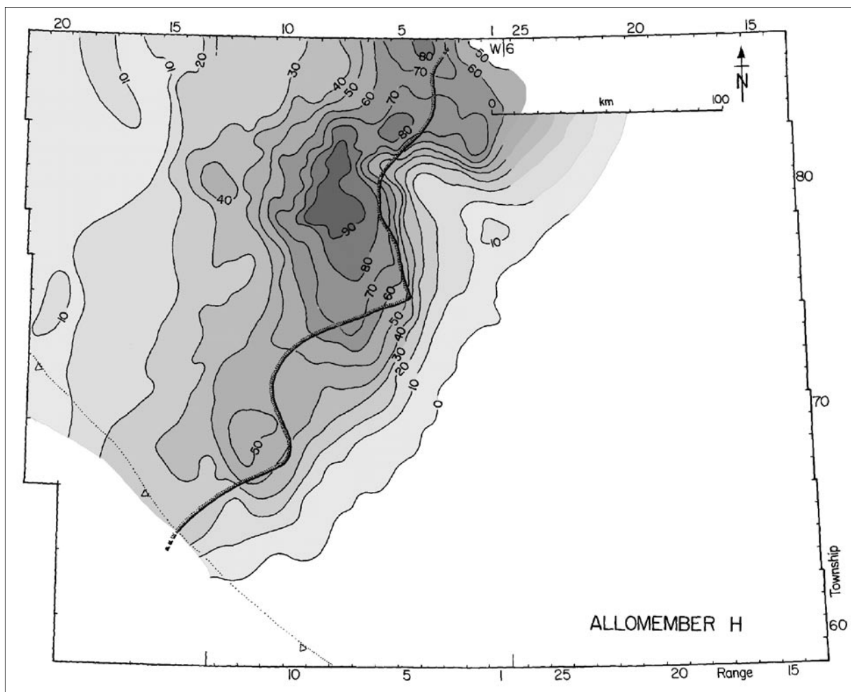
Fig. 12 Palaeogeographic and isopach map of Dunvegan allomember H (from PLINT et al., 2001).
