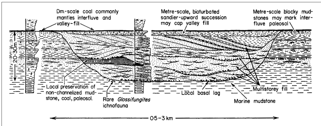
Fig. 18 Transverse section summarizing the main characteristics of valley-fills in an up-valley, fluvial-dominated reach (from PLINT & WADSWORTH, in review).
