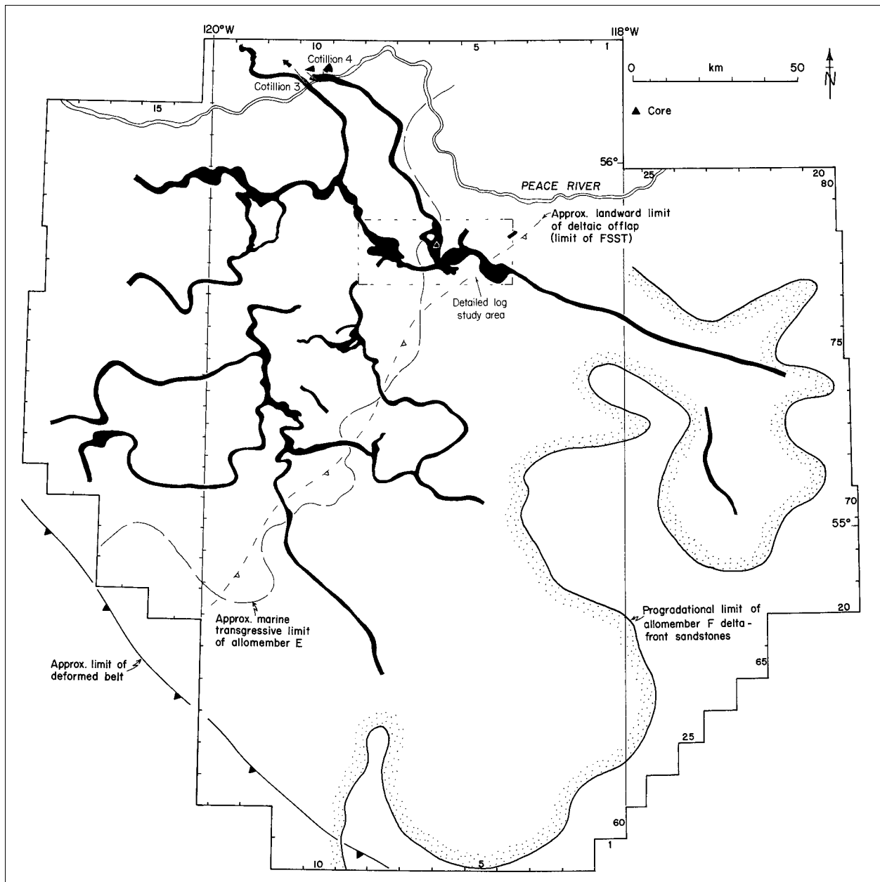
Fig. 27 Palaeogeographic map of allomember F showing the maximum progradational limit of the marine shoreline, the boundary between aggradational (HST) and offlapping (FSST) parasequences, the distribution of valleys, and the maximum transgressive limit of the succeeding allomember E shoreline (from PLINT & WADSWORTH, in review).
