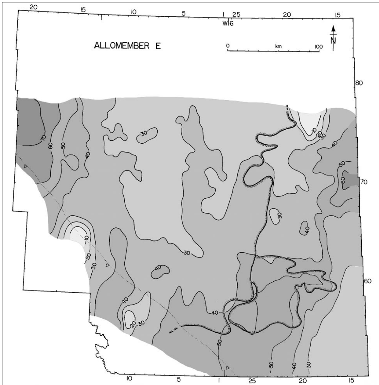
Fig. 15 Palaeogeographic and isopach map of Dunvegan allomember E. Note the appearance of a semi-circular depocentre in the NW corner of the study area, interpreted to record the onset of renewed flexural subsidence (from PLINT et al. , 2001).
