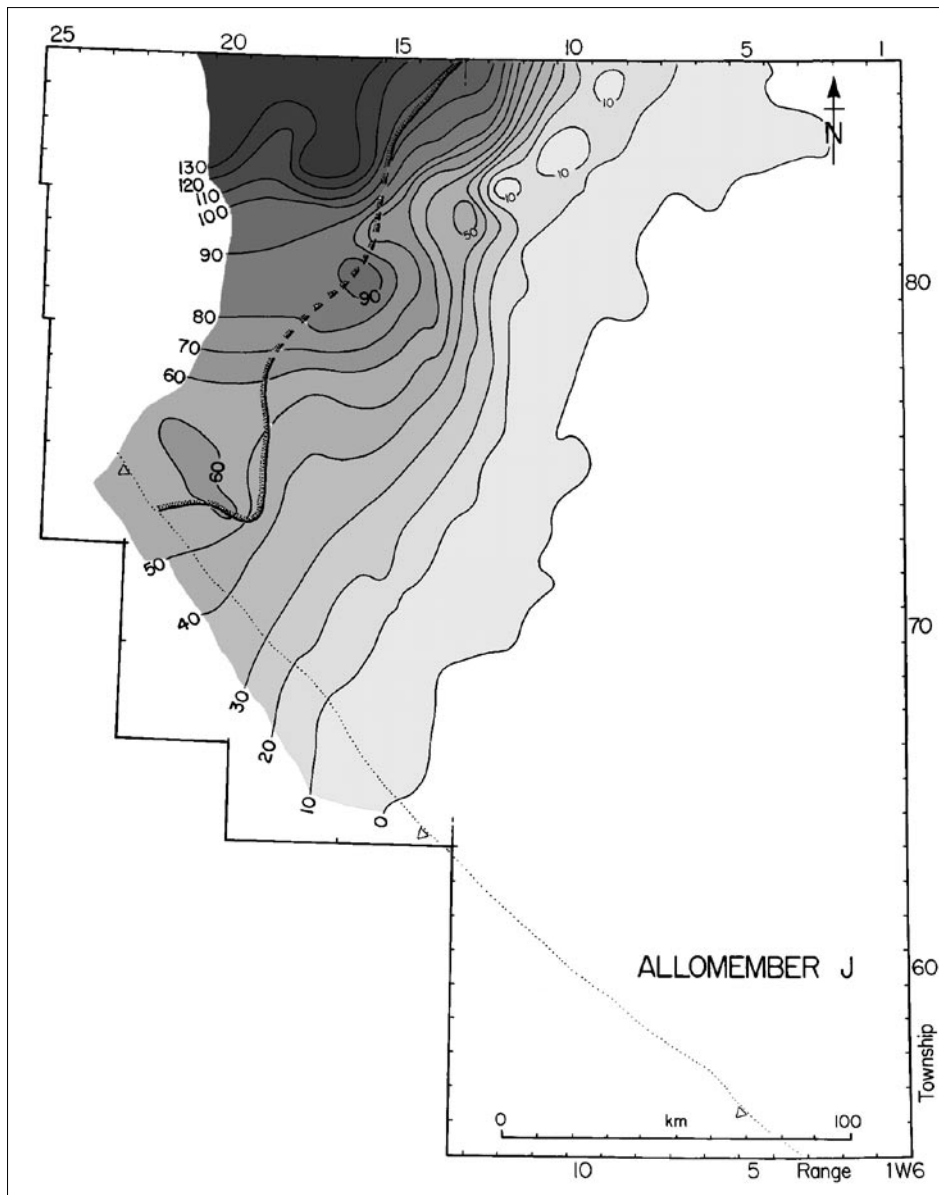
Fig. 10 Palaeogeographic and isopach map of Dunvegan allomember J. Heavy stippled line in this and figures 11–16 indicate the maximum progradational extent of the delta-front sandstone, mapped from gamma ray log signatures. Note how isopach lines trend perpendicular to the orogen in this map and in Figs. 11–14. This pattern is interpreted to reflect deposition at a time when the rate of flexural subsidence was negligible. Contour interval in figures 10–16 = 10 m.
