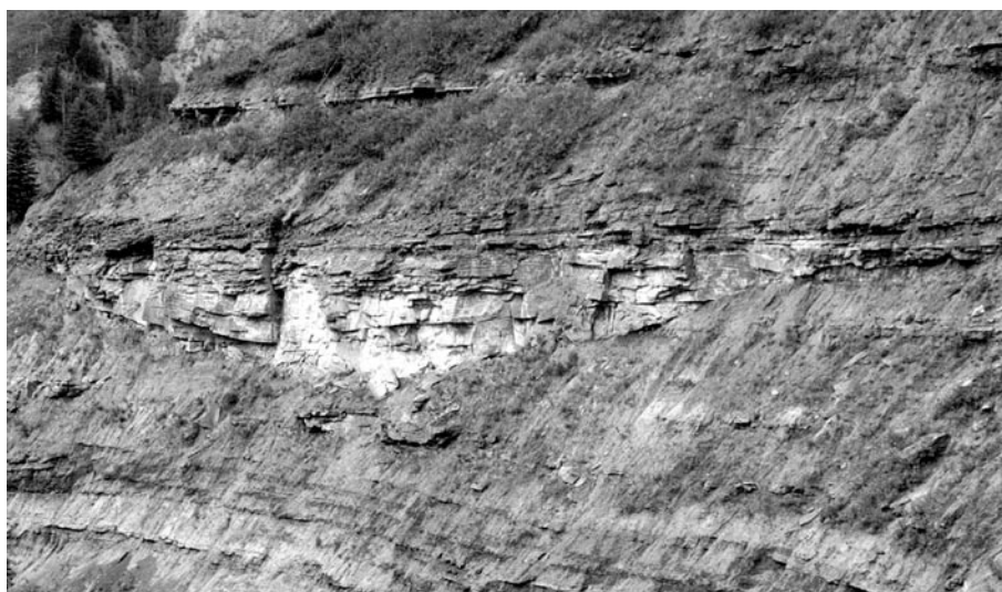
Fig. 20 Example of lenticular fluvial sandstone (up to 8 m thick), interpreted to represent an anabranch of an anastomosed river, enclosed in grey pedogenic and lacustrine mudstones. Coldstream Creek, B.C.
