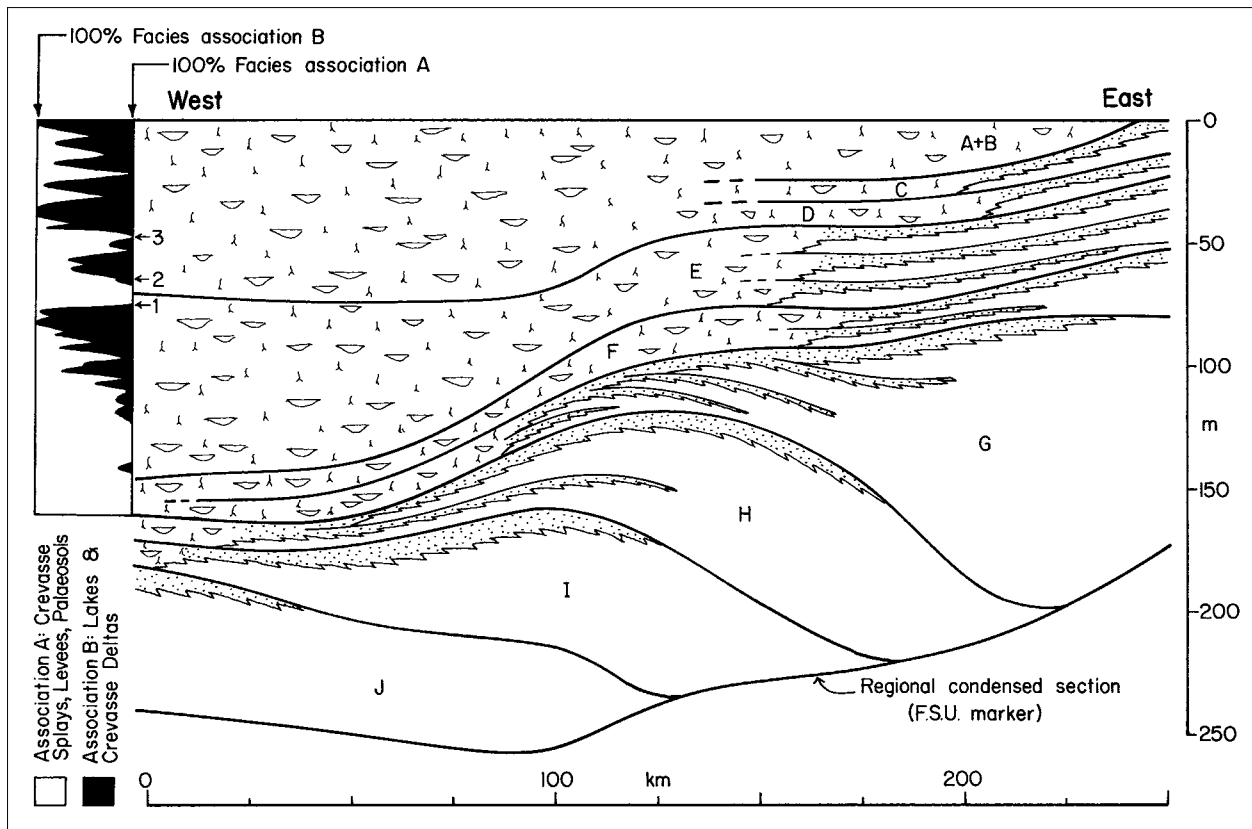
Fig. 26 Summary stratigraphic section oriented E–W across the northern part of the study area (Fig. 1) showing, to scale, the thickness variations of the Dunvegan allomembers. Flexural subsidence was negligible in allomembers J–F, but became increasingly rapid in allomembers E–A as shown by the great expansion of the section towards the west. The increased accommodation rate is reflected in the vertical changes in alluvial facies in outcrop, with an overall upward increase in the proportion of waterlogged and subaqueous facies (association B) relative to better-drained facies (association A; from LUMSDON & PLINT, 2003).
