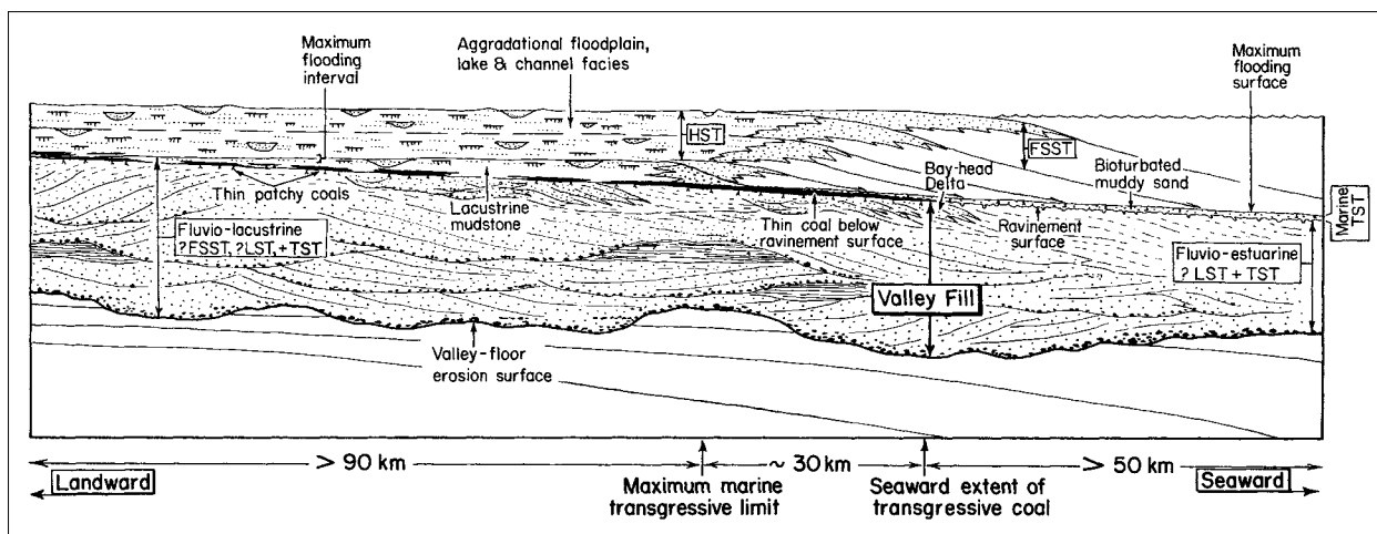
Fig. 19 Longitudinal section summarizing the main characteristics of valley-fills from the valley mouth to a point about 180 km up-valley (from PLINT & WADSWORTH, in review).
