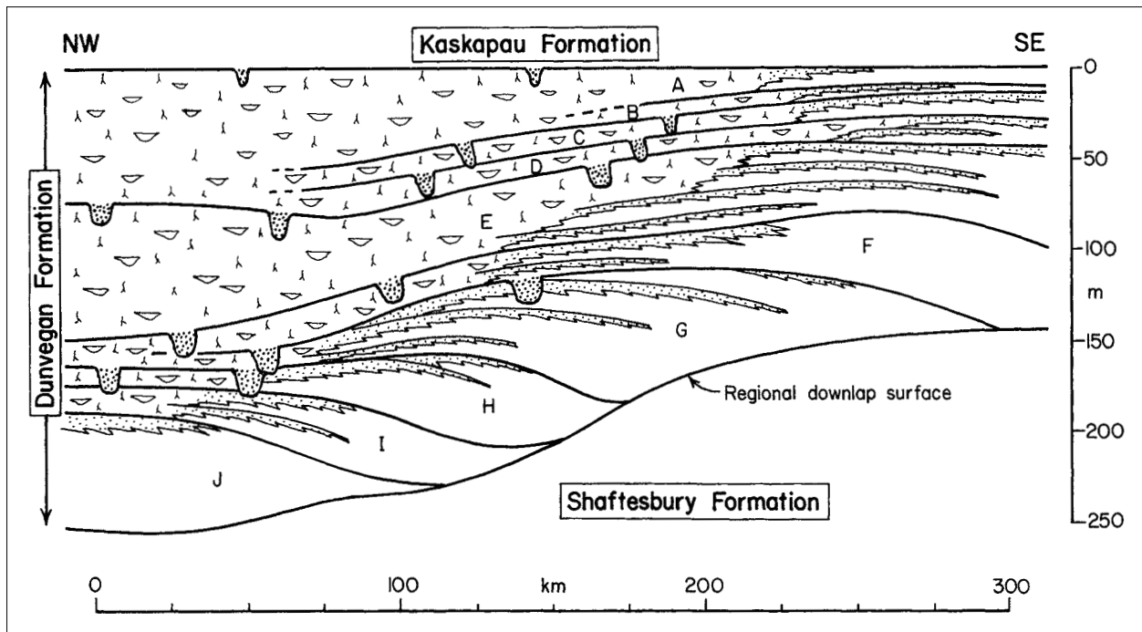
Fig. 23 Summary dip section (located in Fig. 1) drafted to scale, with the top of allomember A as a datum, showing the stratigraphic distribution of valley-fills. Only valleys on allomembers H–E can be mapped with the available well density (from PLINT & WADSWORTH, in review).
