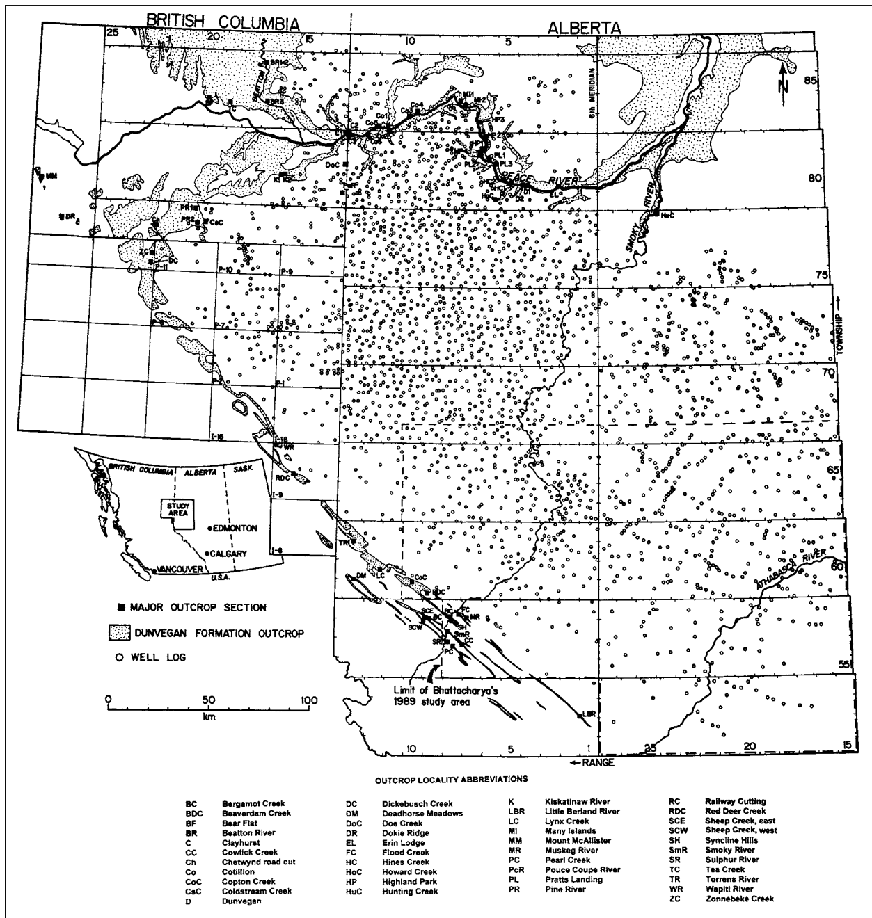
Fig. 2 Map of study area showing stratigraphic data base, including location of 2340 well logs and principal outcrop sections in the Foothills and Peace River valley (from PLINT, 2000).
