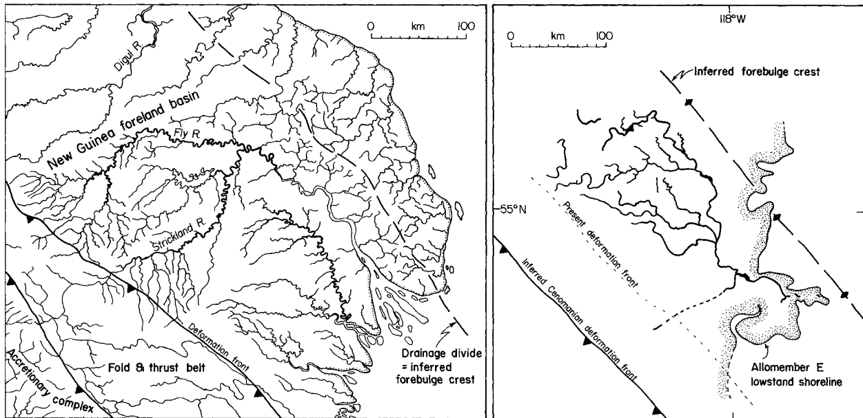
Fig. 30 Maps comparing the pattern, scale and palaeogeographic relationships of the modern Fly River (flipped and rotated) so as to mimic the orientation of the valley system in Dunvegan allomember E.
