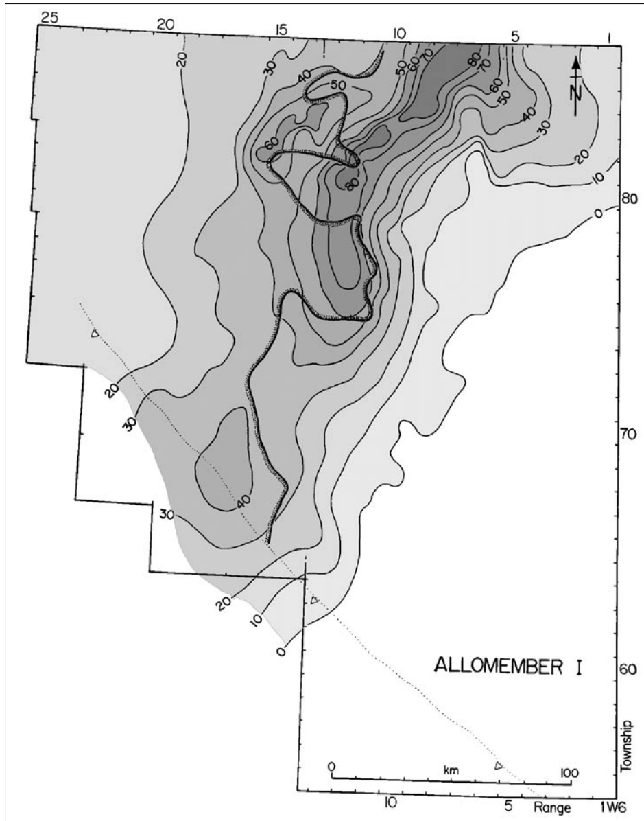
Fig. 11 Palaeogeographic and isopach map of Dunvegan allomember I.
