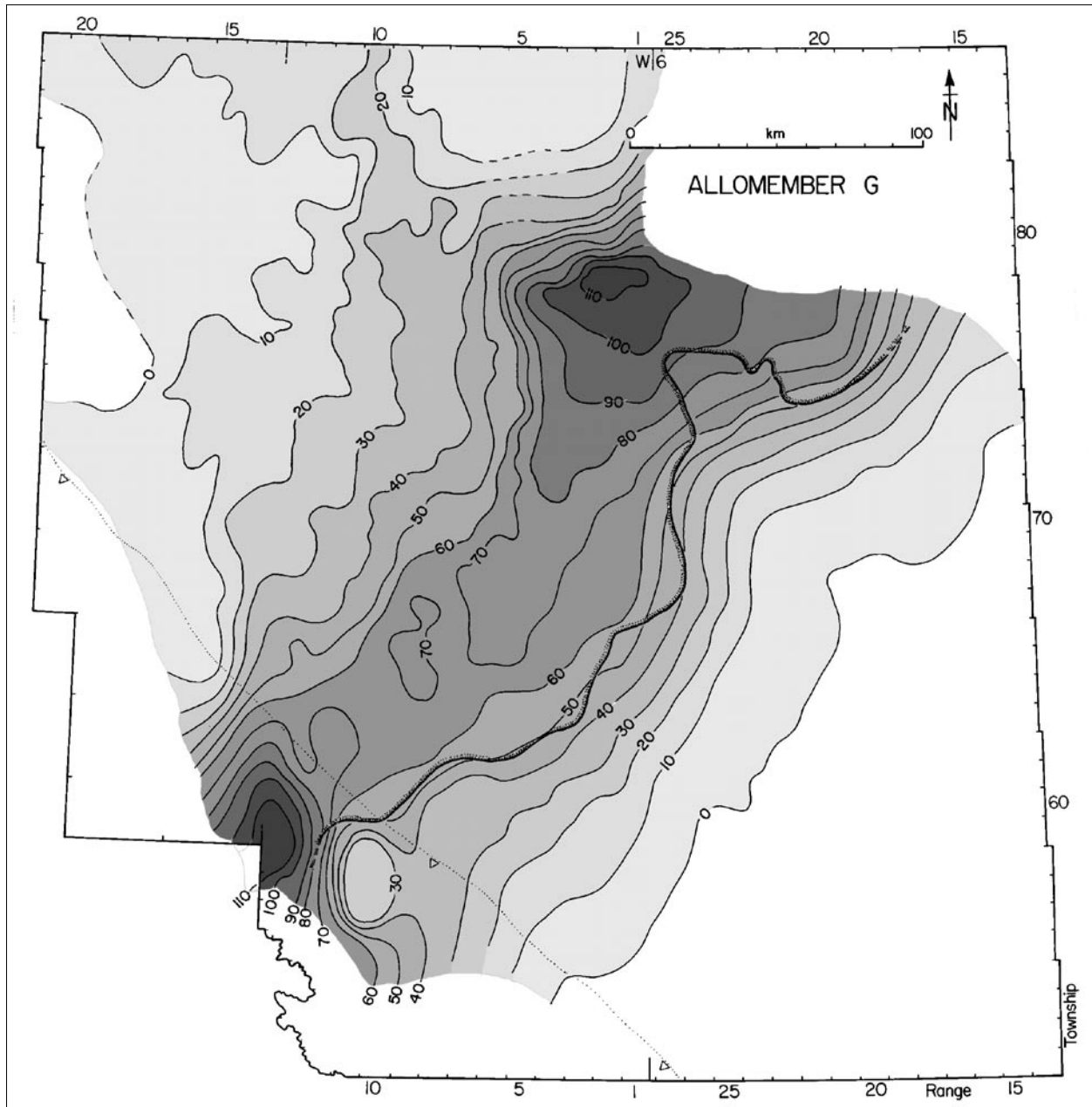
Fig. 13 Palaeogeographic and isopach map of Dunvegan allomember G (from PLINT et al., 2001).
