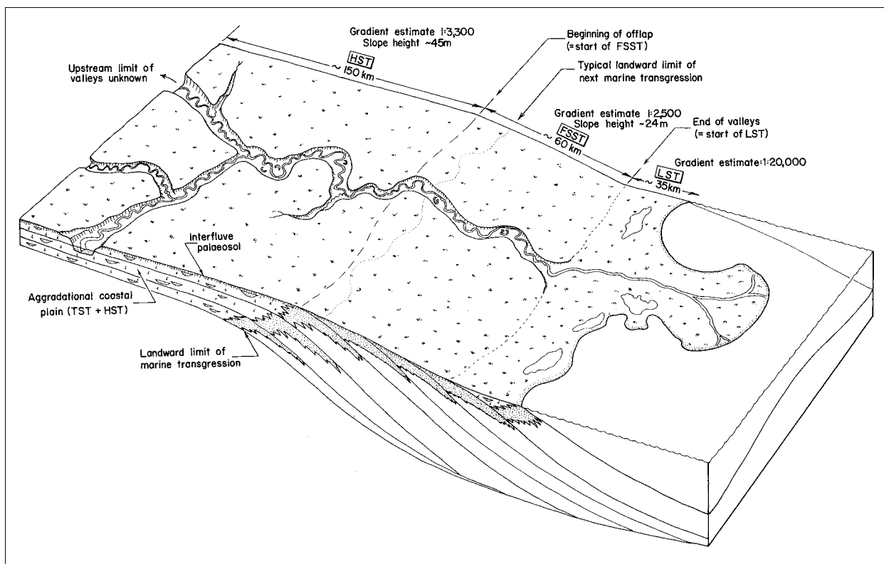
Fig. 31 Block diagram summarizing the stratigraphic, geographic and topographic relationships between valleys and various systems tracts of a delta complex. Strata assigned to the TST and HST include aggradational coastal plain deposits. Offlapping deltaic strata of the FSST lack coeval coastal plain deposits and prograde an average of 60 km during slow relative sea level fall. Fluvial incision is inferred to have occurred during this time, and was accompanied by development of very mature interfluvial palaeosols. Valley systems generally terminate about 35 km from the maximum progradational limit of the delta front, and this limit is interpreted to indicate the FSST/LST boundary. Aggradational and onlapping LST strata average 35 km wide, but include major lowstand deltas constructed at the termini of valley systems. On the basis of the assumed slopes and measured geographic dimensions, it is possible to infer cyclic eustatic changes of about 24 m (see text for discussion) (from PLINT & WADSWORTH, in review).
