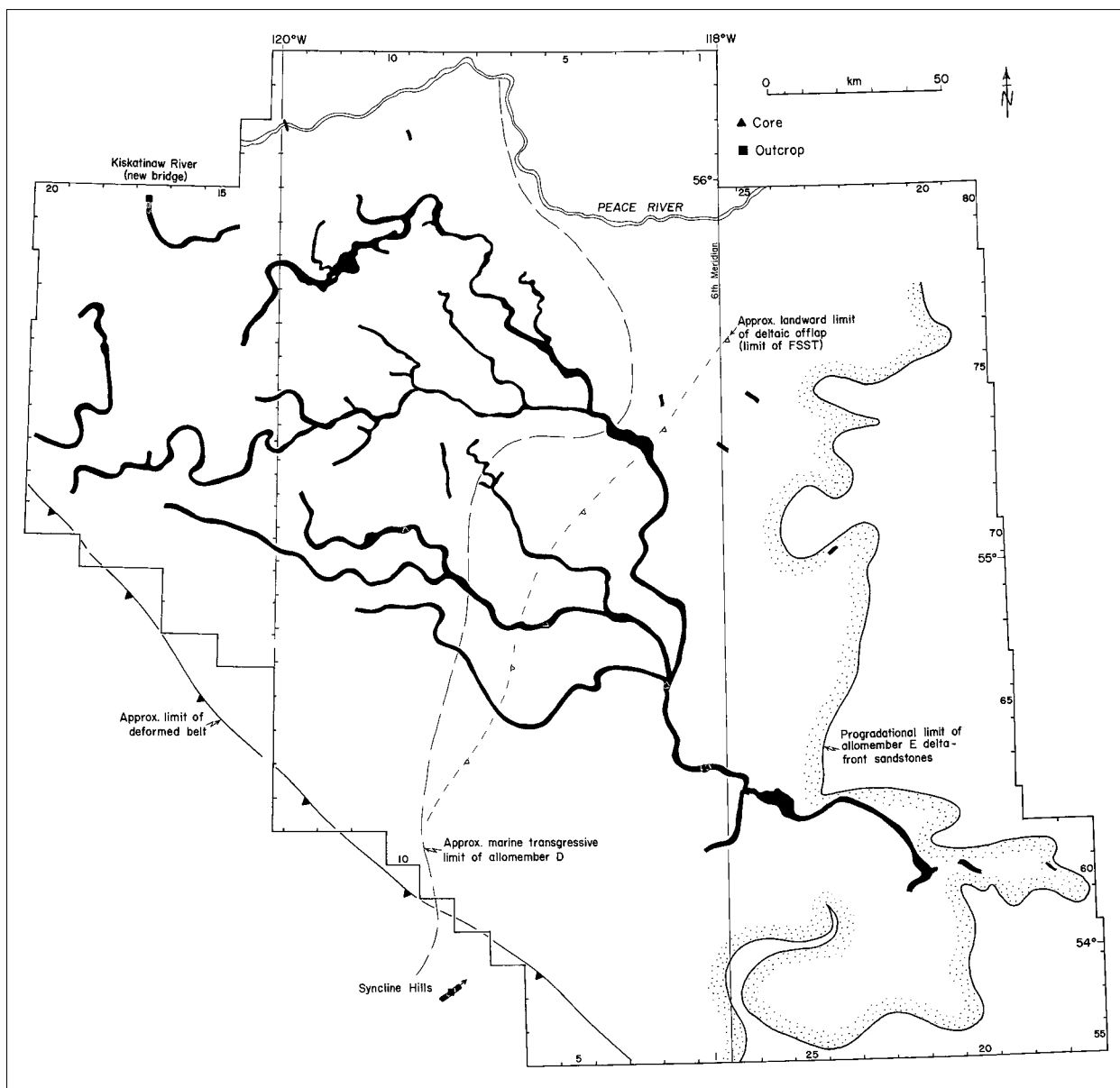
Fig. 28 Palaeogeographic map of allomember E showing the maximum progradational limit of the marine shoreline, the boundary between aggradational (HST) and offlapping (FSST) parasequences, the distribution of valleys, and the maximum transgressive limit of the succeeding allomember D shoreline (from PLINT & WADSWORTH, in review).
