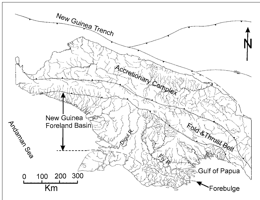
Fig. 29 Map of rivers in the central portion of the New Guinea foreland basin. The distinct drainage divide close to the southern coast is interpreted to reflect the position of the forebulge. Note how the Fly and Digul river systems flow initially perpendicular to the fold and thrust belt, but distally, are diverted by and flow parallel to the forebulge.
