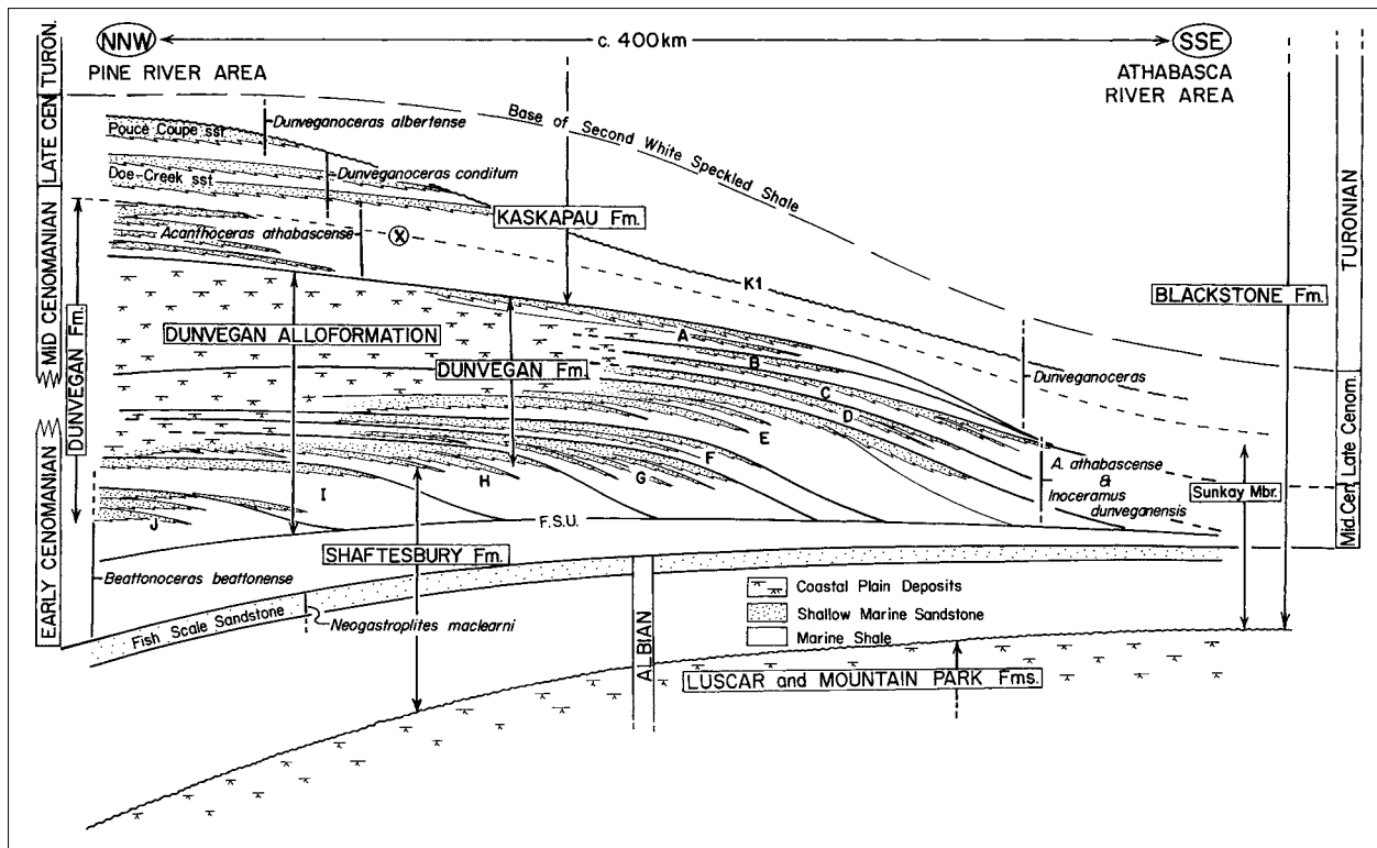
Fig. 3 Schematic NW-SE dip section showing the Dunvegan Fm., the stratigraphic terminology applied to the under- and overlying units, and the stratigraphic range of important Zone fossils. The boundaries of the lithostratigraphic Dunvegan Fm., and the allostratigraphic Dunvegan alloformation are also indicated. The former is very diachronous (from PLINT et al., 2001).
