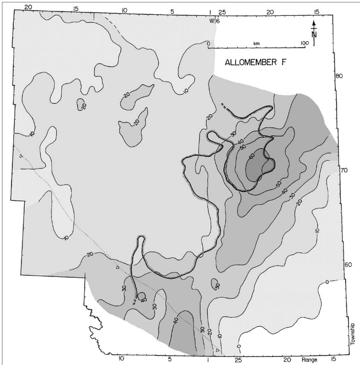
Fig. 14 Palaeogeographic and isopach map of Dunvegan allomember F (from PLINT et al., 2001).
