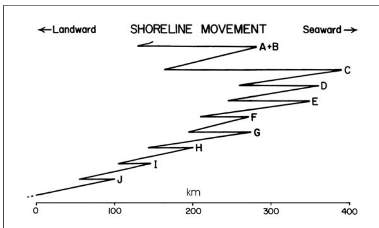
Fig. 24 Scale drawing summarizing the average shoreline displacement for each transgressive–regressive cycle of the Dunvegan Fm. Note the similarity in shoreline displacement for allomembers I–C. Only the transgressions at the tops of allomembers C and A show a transgressive distance that greatly exceeds the regressive distance, probably reflecting an accelerating subsidence rate and increasing accommodation: sedimentation ratio (see also Fig. 16).
