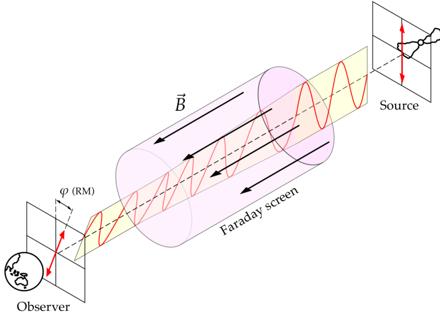
Figure 2.2: The Faraday effect for a single Faraday screen with magnetic field \vec{B} inducing a Faraday rotation of \phi . Adapted from a figure by Bob Mellish.
