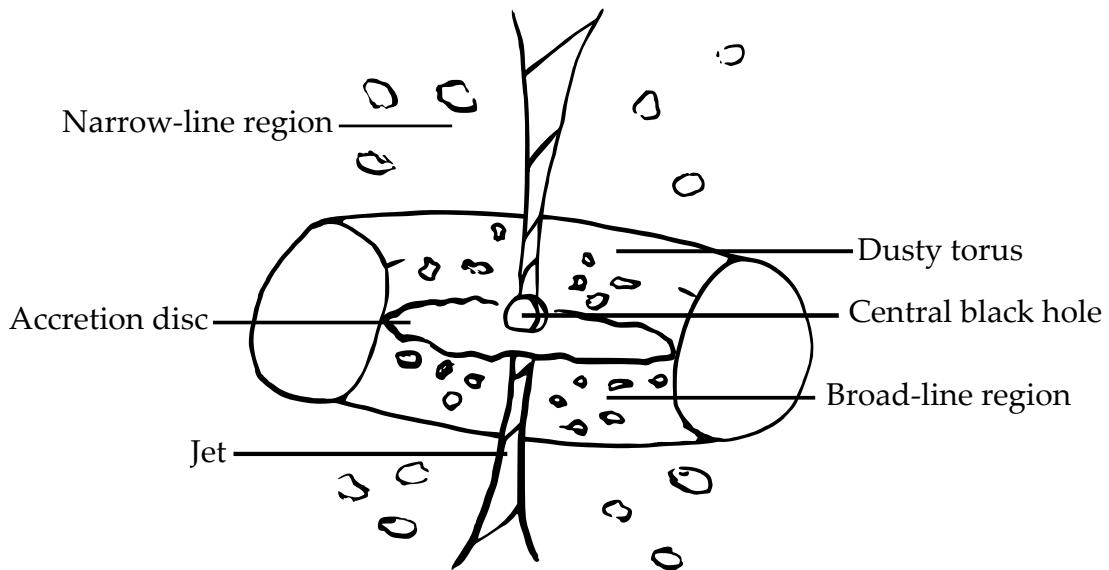
Figure 2.5: The unified model of AGN.
