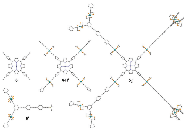
Fig. 3 Optimized structures of 6 (top left), 4-H' (middle), 5 2 ' (right) and 9' (bottom left). Hydrogen atoms are omitted for clarity.
