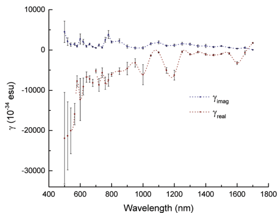
Fig. 7 Plots of the real (red) and imaginary (blue) components of the second hyperpolarizability for 5 2 .
