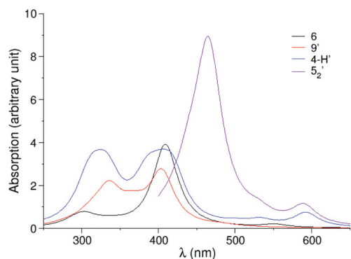
Fig. 5 Calculated UV-vis absorption spectra of the compounds 4-H' , 5 2 ' , 6 , and 9' . Computations were carried out up to 400 nm for 5 2 ' due to computational limitations.
