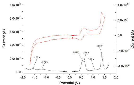
Fig. 1 Cyclic voltammogram (in red) of the zinc porphyrin 5 2 in THF/ [\text{NBu}_4][\text{PF}_6] (0.1 M) at 25 °C at 0.1 V s -1 between -1.6 and 1.4 V vs. SCE. The differential pulse voltammetry (DPV) trace (in black) is drawn below the cyclic voltammogram.
