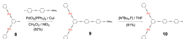
Scheme 1 Synthesis of the wedge 10 .
