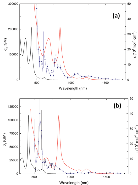
Fig. 8 Two-photon absorption cross-section plots for 5 2 (a) and 7 (b) with trendline as a visual aid (blue) overlaid on one-photon absorption (OPA) spectra (black) and the same OPA plotted at twice the wavelength.
