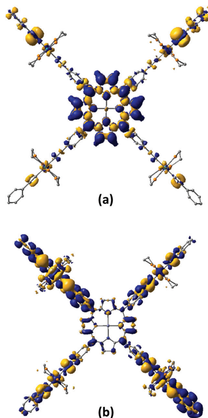
Fig. 6 Density-difference plot associated with (a) the Soret band and (b) the MLCT band \lambda = 332 nm in 4-H' . The blue and yellow colours indicate an increase and decrease of density upon excitation, respectively [isocontour value = 0.0002 e bohr -3 ].
