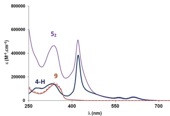
Fig. 2 UV-vis absorption spectra of the zinc(II) porphyrin 4-H and 5 2 and of the organometallic wedge 9 in \text{CH}_2\text{Cl}_2 at 25 °C.
