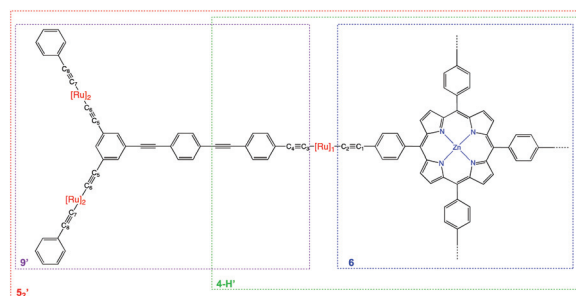
Fig. 4 Atom labeling in compounds 4-H' , 5 2 ' , 6 and 9' ([Ru] = Ru (dpe) 2 ).
