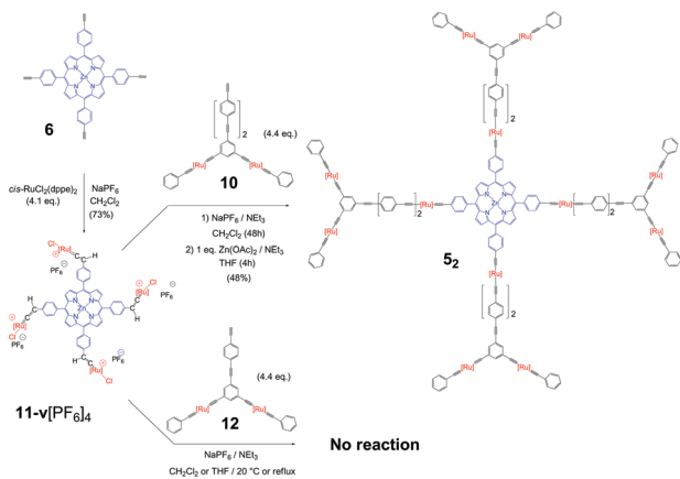
Scheme 2 Synthesis of 5 2 .
