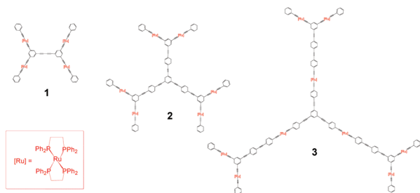
Chart 1 Some Ru(II)-containing organometallic dendrimers developed for cubic optical nonlinearity.
