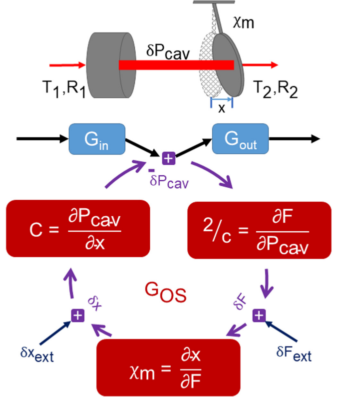
FIG. 2. Detailed loop diagram for the cavity's transfer function. The amplitude modulator adds to the intracavity power P_{cav} . The cavity power converts into radiation pressure force F , which then converts into cantilever displacement x via its mechanical susceptibility \chi_m . The displacement causes a length change for the cavity, leading again to a change in the intracavity power via the cavity response C . This forms a closed-loop system.
