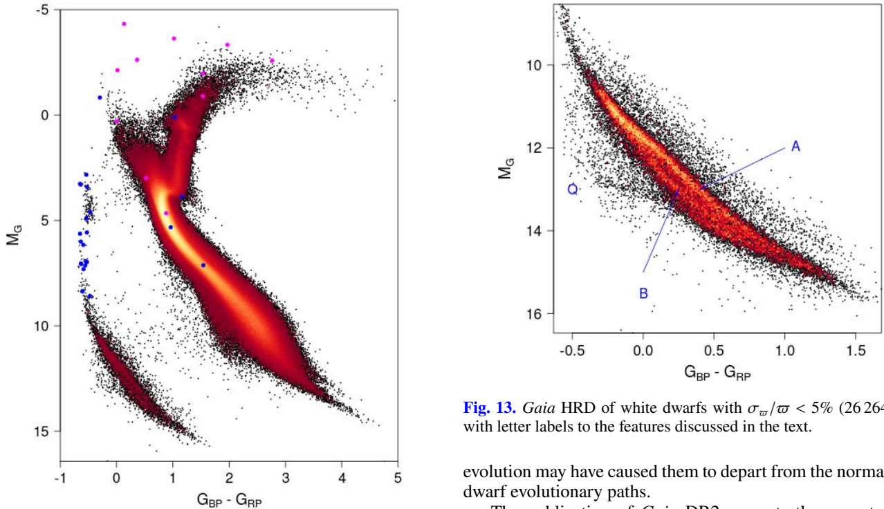
Fig. 12. North Galactic Pole HRD ( b > 50^\circ , 2 077 925 stars) with literature central planetary nebula stars (blue) and post-AGB stars (magenta).
