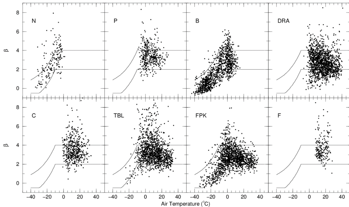
Figure 2. Variation of \beta (derived from radiosonde data) for selected sites. Site ids (Table 1) are given in each panel. The upper line in each panel corresponds to the estimated value of \beta for clear sky conditions, and the bottom line shows the value for A_c=1 .
