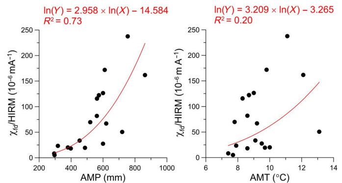
Fig. 3. \chi_{fd}/HRM versus annual mean precipitation and temperature for surface soil samples across the CLP. The annual mean temperature (AMT) and the annual mean precipitation (AMP) data are from meteorological stations on the CLP. The sample sites are the same as those in the study by Nie et al. (85).
