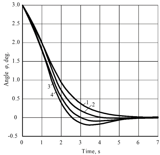
Figure 3. Dynamics of change in the disk harrow deviation angle \varphi at different forward speeds V_0 : 1 – V_0 = 2.86 \text{ m s}^{-1} ; 2 – V_0 = 3.36 \text{ m s}^{-1} ; 3 – V_0 = 3.86 \text{ m s}^{-1} ; 4 – V_0 = 4.36 \text{ m s}^{-1} .
