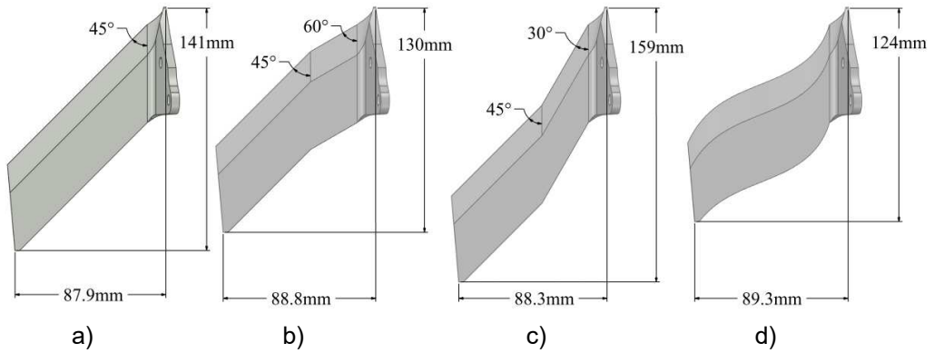
Figure 2. Schema of wings types: a) type 0 b) type 1 c) type 2 d) type 3.
