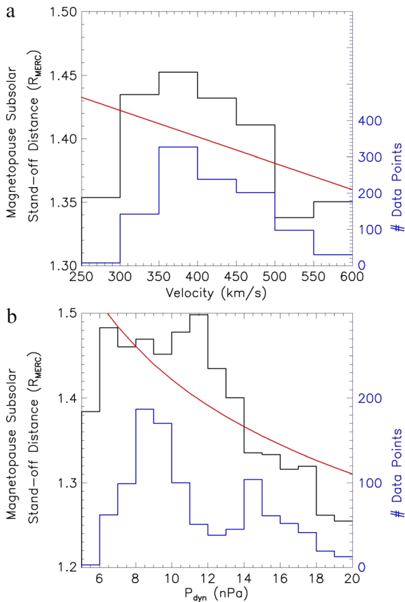
Figure 11. (a) Relation between mean magnetopause standoff distance (in units of Mercury radii, R_M ) and solar wind velocity (computed by ENLIL). The red line shows the linear least squares fit of the mean R_{ss} values versus V . The blue histogram (axis to the right) shows the number of magnetopause location values for each solar wind speed interval in the black histograms. (b) Relation between mean magnetopause standoff distance and solar wind dynamic pressure ( P_{dyn} ) computed by ENLIL. The red curve shows the expected P_{dyn}^{-1/6} dependence of R_{ss} (see text).
