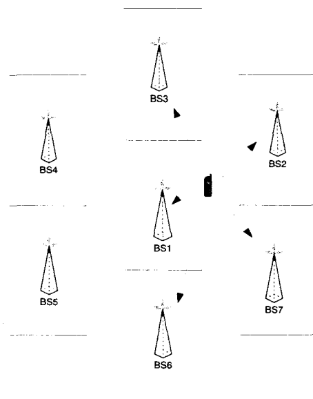
FIGURE 2.1 A TYPICAL PL SYSTEM IN CELLULAR NETWORK
