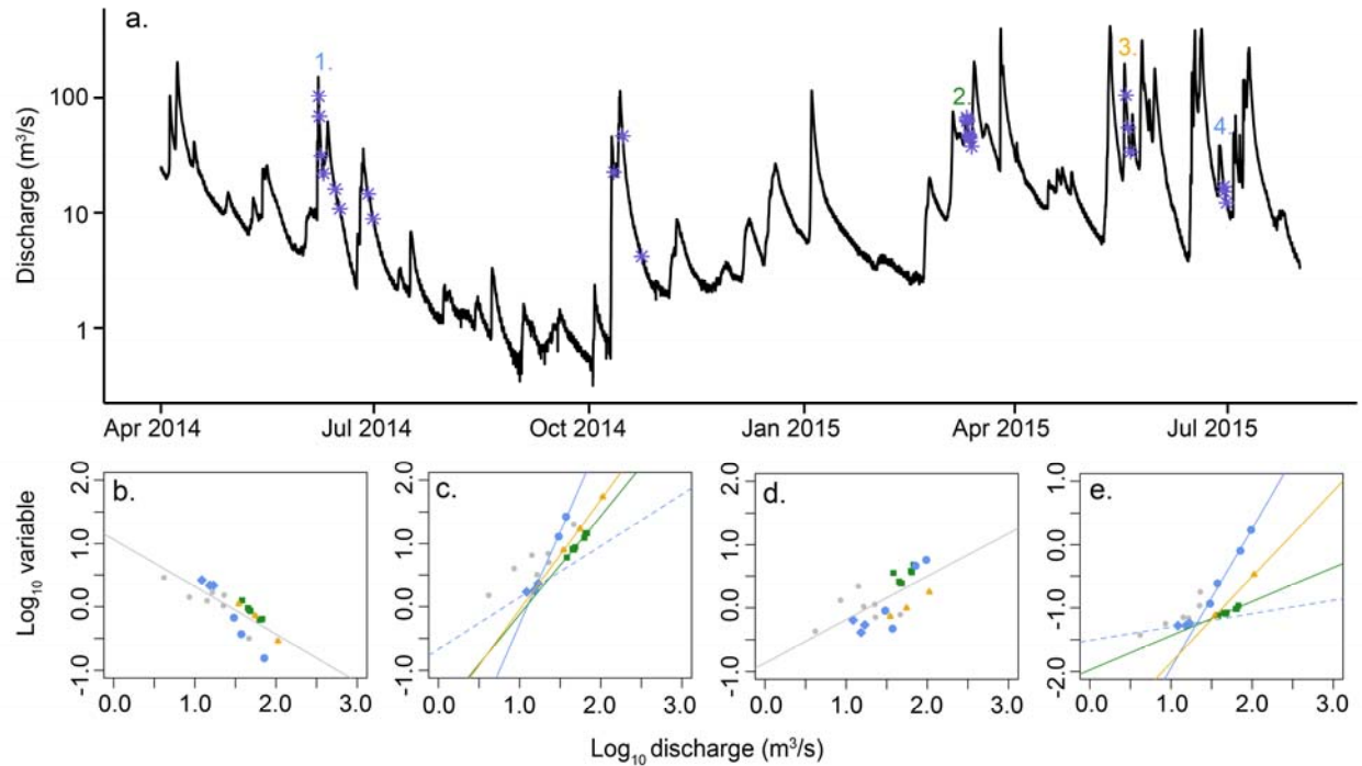
Figure 5. Kings River hydrograph (a) and ordinary least squares regression results of \log_{10} transformed water quality variables versus \log_{10} transformed discharge ( \text{m}^3/\text{s} ); b) black disk visibility (m); c) total suspended solids (mg/L); d) suspended chlorophyll- \alpha (mg/L); e) particulate nitrogen (mg/L); multiple lines indicate significant interaction effects (ANCOVA); dashed lines indicate the regression slope was not significantly different from zero.
