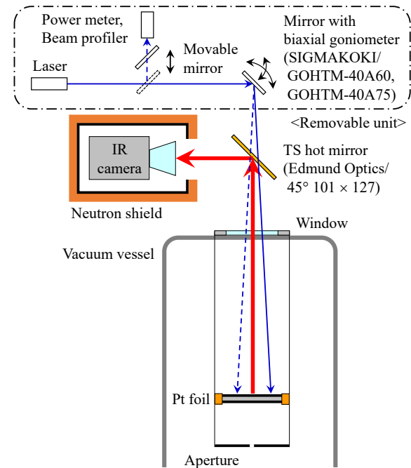
FIG. 1. (Color online). Schematic of the in-situ calibration system for the thermal characteristics of the IRVB foil.
