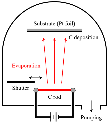
FIG. 2. (Color online). Schematic of evaporation coating.
