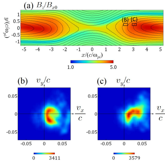
FIG. 8: Simulation results for the case of B_{z0}/B_{x0} = 3.0 . (a) Spatial profile of magnetic field lines and B_z/B_{x0} . (b) Ion velocity distribution at the boxed area (B). (c) Ion velocity distribution at the boxed area (C). Crescent-like structures are formed.
