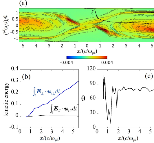
FIG. 5: (a) Profiles of \mathbf{E} \cdot \mathbf{u}_i , (b) the integral of the perpendicular (the blue line) and parallel (the black line) components of \mathbf{E} \cdot \mathbf{u}_i , and (c) the angle between \mathbf{E}_{\perp} and \mathbf{u}_{i\perp} along the streamline \ell [the dotted line of the panel (a)]. Ions gain kinetic energy from \mathbf{E}_{\perp} not only on the separatrix but also in the downstream. It is of interest that \mathbf{u}_{i\perp} is nearly parallel to \mathbf{E}_{\perp} on the separatrix and is nearly perpendicular to \mathbf{E}_{\perp} in the downstream. The electric field, the velocity, and the time are normalized to B_{x0} , c , and \omega_{pi}^{-1} , respectively.
