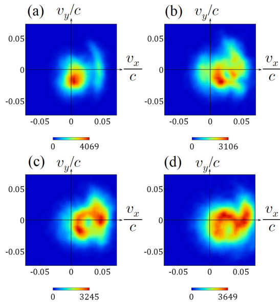
FIG. 3: Ion velocity distributions at the local regions (A)-(D) of Fig. 1. The panels (b) and (c) show ring-like structures.
