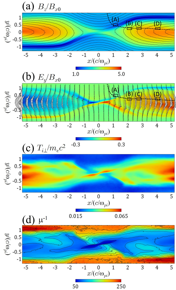
FIG. 2: Spatial profiles of (a) magnetic field lines and B_z , (b) ion bulk velocity vectors and E_y , (c) ion temperature perpendicular to the magnetic field, and (d) average of inversed ion magnetic moments. The electromagnetic field, the velocity, and the temperature are normalized to B_{x0} , c , and m_e c^2 , respectively.
