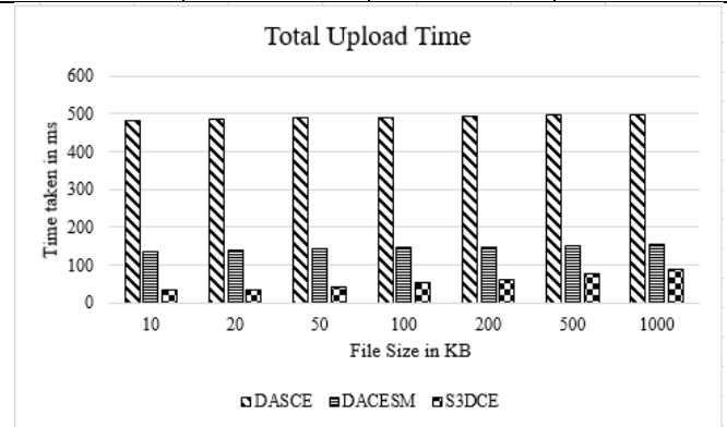
Fig 3: Comparison of Total Upload Time of DASCE, DACESM, S 3 DCE
