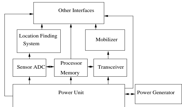
Fig. 1: Sensor Node Hardware
