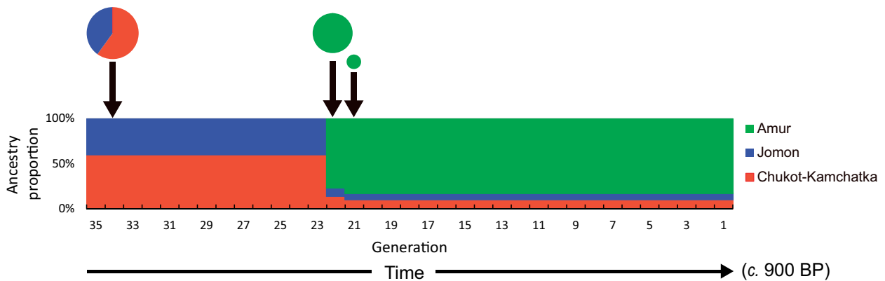
FIG. 7. —Migration model inferred from the tract length distributions. The single pulse model of three populations was assumed. 0 generation corresponds to the 14 C age of NAT002 (~900 BP).
