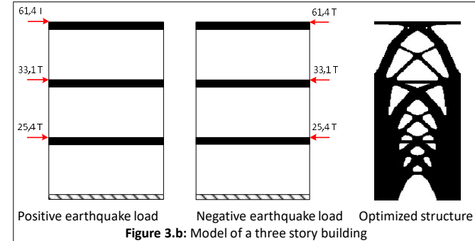
Figure 3.b: Model of a three story building
