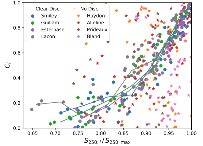
Figure 5. Cosine similarity C against S_{250} flux density (observer-frame), normalised to the maximum of the 50 orientations. Galaxies with clear disc morphologies (Smiley, Guillem, Esterhase, Lacon; circular markers) show a clear positive correlation, further emphasised by the lines which show the binned medians, whereas galaxies without a disc (Haydon, Alleline, Prideaux, Bland; star markers) show no such relationship.
