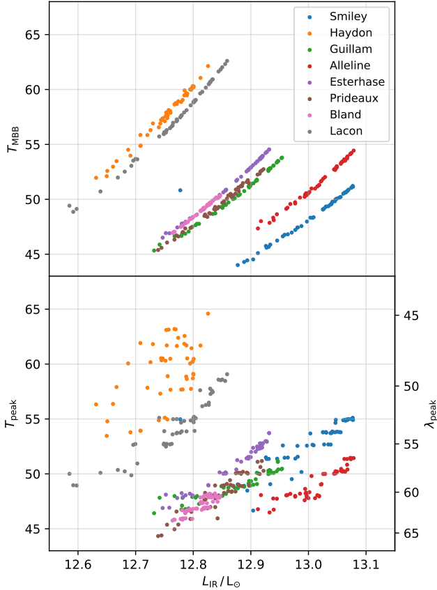
Figure 6. Distribution of estimates of temperature and FIR luminosity for all 50 orientations of our eight sub-mm galaxies. Top: Temperature ( T_{\text{MBB}} ) and L_{\text{IR}} estimated through MBB fits to the sub-mm emission. Bottom: The temperature estimate from the peak of the SED in the FIR regime ( T_{\text{peak}} ).
