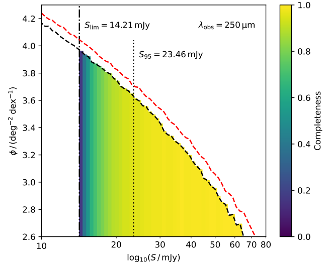
Figure 8. The observed S_{250\mu\text{m}} number count distribution from our model. The red dashed line shows the number counts before dimming is applied, the black dashed line shows the counts after dimming. The dimmed counts are coloured by the orientation completeness, for a flux-density limit S_{\text{lim}} = 14.21 \text{ mJy} (dashed-dotted line). The flux density at which the completeness is 95% ( S_{95} = 23.46 \text{ mJy} ) is shown by the dotted line. The completeness at a given flux density is dependent on both S_{\text{lim}} and wavelength.
