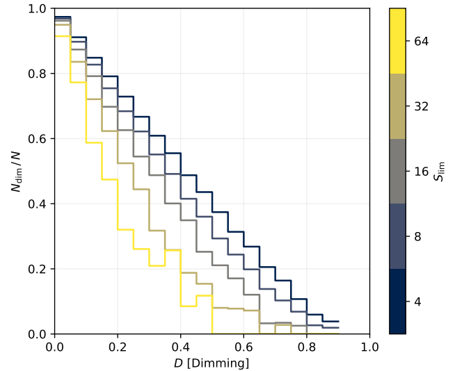
Figure 9. Fraction of galaxies recovered, binned by dimming D , at \lambda_{\text{obs}} = 250 \mu\text{m} . Each coloured line shows a different flux density limit ( S_{\text{lim}} ). As expected, the most dimmed galaxies (due to a combination of morphology and orientation) are less likely to be detected, and this effect is strongest for higher S_{\text{lim}} .
