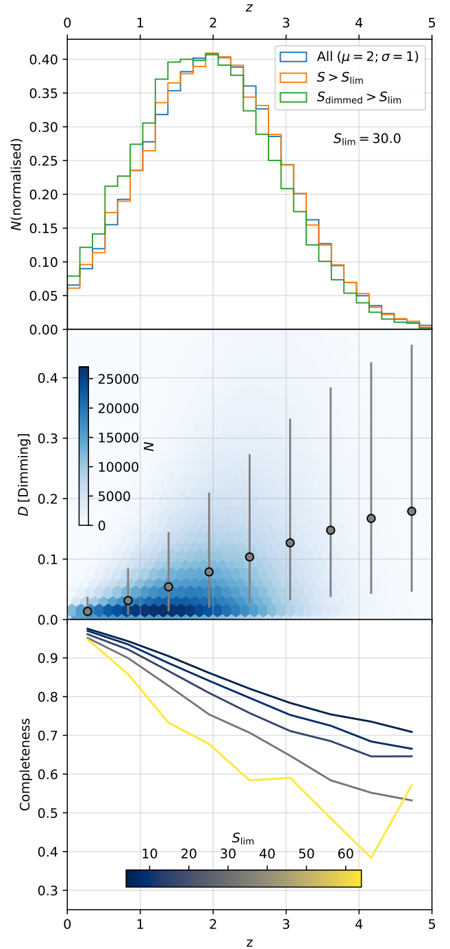
Figure 10. Redshift distribution of sources in a mock 250 \mu\text{m} survey. Top: The normalised redshift distribution of all sources (blue), those whose un-dimmed flux density is above S_{\text{lim}} = 30 (orange), and those whose dimmed flux density is above S_{\text{lim}} . There is a slight bias towards lower redshifts as a result of the orientation-dependent dimming. Middle: the distribution of dimming values for the mock galaxies. Grey points show the median distribution binned in redshift, with errors showing the 16 th –84 th percentile range. The 2D histogram (blue) shows the distribution of all sources. Galaxies at higher redshift are more likely to experience high orientation-dependent dimming. Bottom: completeness as a function of redshift z at a given S_{\text{lim}} . The redshift-dependent dimming leads to a redshift-dependent incompleteness.
