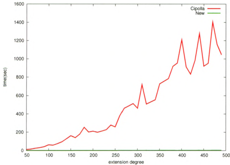
Figure 6.1: The new square root algorithm
