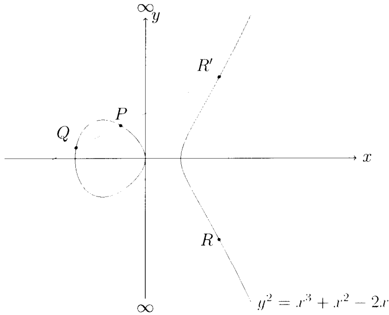
Figure 2.1: P + Q = R
