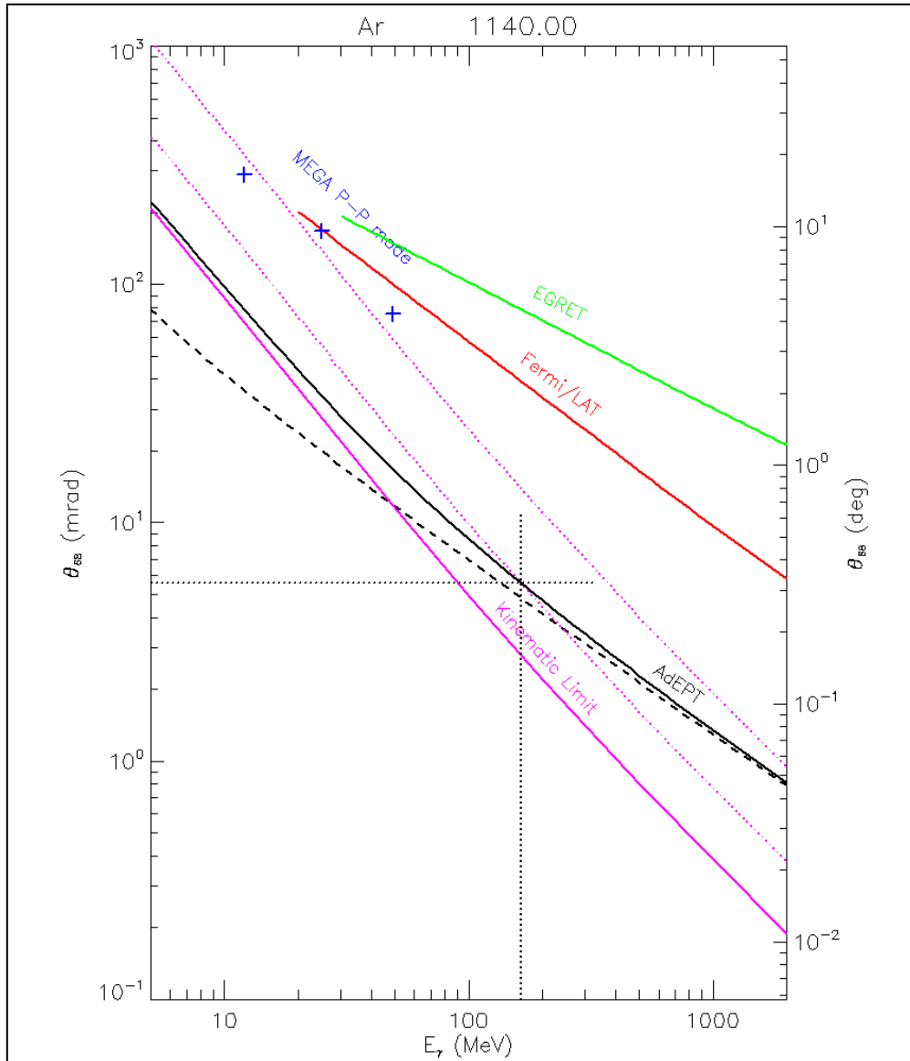
Figure 1 - The calculated angular resolution of the AdEPT telescope concept (solid black line, see §6 and Table 3) as a function of the gamma ray energy is the quadrature sum of the kinematic limit determined for nuclear pair production from [19] (solid magenta line) and the angular resolution limited only by MCS of the electron-positron pair (black dashed line). Twice, and five times the kinematic limit is also shown (dotted magenta lines). Below ~200 MeV, the AdEPT telescope will achieve angular resolution within a factor two of the kinematic limit. The MEGA [29] measured pair production angular resolution (blue crosses), EGRET [73] calibrated angular resolution (green line), and Fermi/LAT front [74] on-orbit angular resolution (red line) are shown for comparison.
