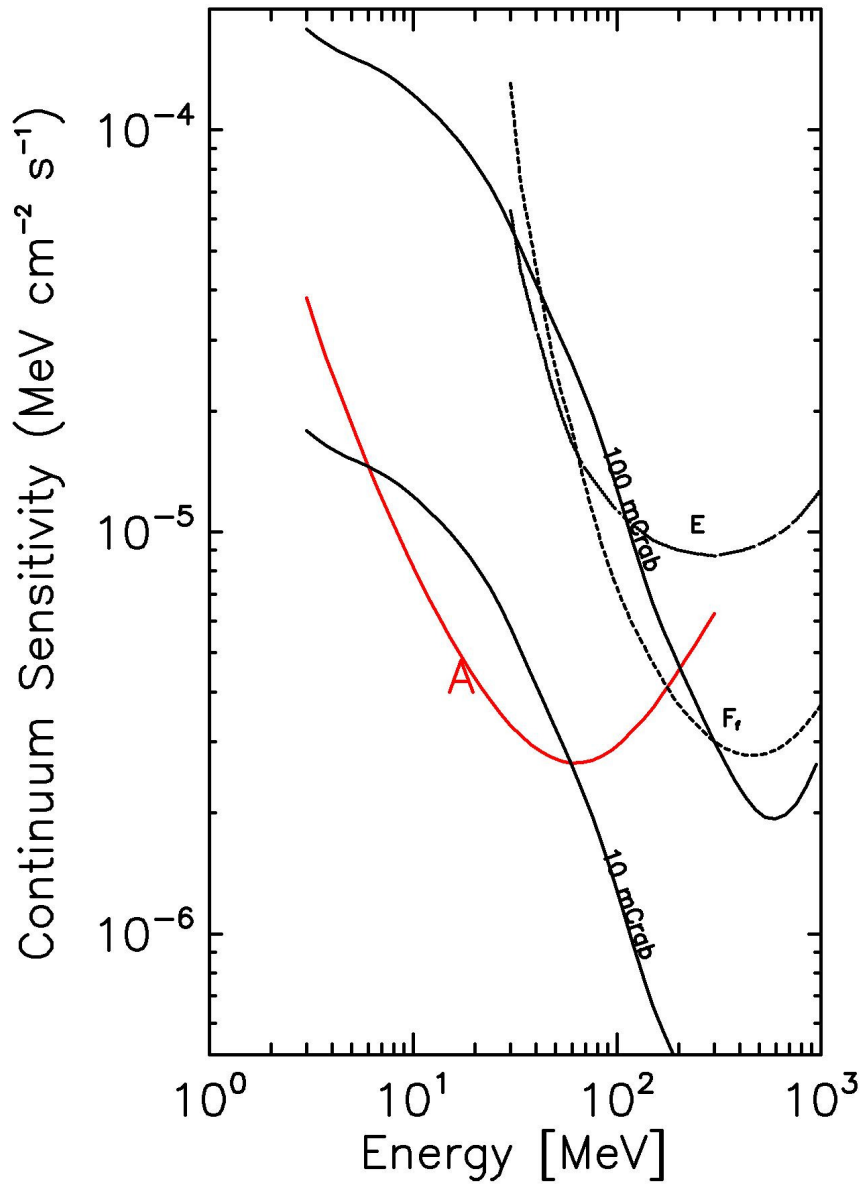
Figure 9 - Continuum sensitivity of the AdEPT instrument concept (Table 3) (A, solid red lines) calculated on the assumption of 3\sigma significance, T_{\text{obs}}=10^6 s, \Delta E=E , and F_{\text{egb}}=2.7\pm 10^{-3} (E/1 MeV) -2.1 . The sensitivity of EGRET (E, dotted black lines), FERMI-LAT front detector (F r , dashed black lines) calculated on the same assumptions. Spectra corresponding to 100 mCrab and 10 mCrab sources are shown for comparison.
