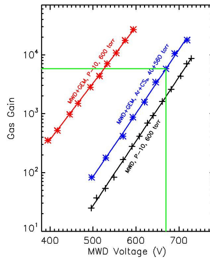
Figure 4 - The gain of our MWD (black data and line) and MWD+GEM (red data and line) as a function of MWD voltage measured in P-10 at 600 torr. The GEM pre-amplifier was operated at a gain of \sim 100 corresponding to a MWD voltage reduction of \sim 200 V. The gain of the MWD+GEM as a function of MWD voltage measured in Ar+CS 2 (blue data and line) shows that gains in excess of 10^4 can be achieved. The nominal operating voltage for the MWD and the total gain are indicated by the green lines.
