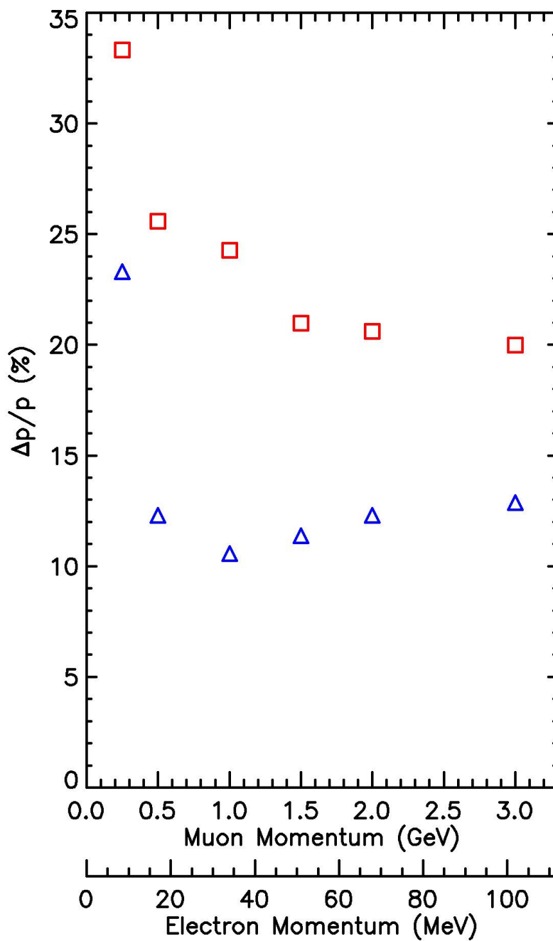
Figure 11 – Monte-Carlo simulation of the ICARUS momentum resolution using classical method (red squares) and the Kalman Filter method (blue triangles). The lower momentum axis has been scaled by the square root of the detector radiation length to give an estimated electron momentum resolution for AdePT. Adapted from [89].
