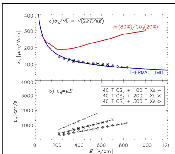
Figure 3 – (top) The longitudinal negative ion diffusion and (bottom) the drift velocity ( v_d = \mu E ) for mixture of Xe + CS 2 . Thermal diffusion limit for T=300 K is shown as the blue line. Non-thermal diffusion for Ar+CO 2 [63] is shown as the red line.
