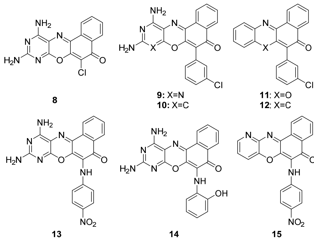
Figure 11. Compound 8 and derivatives obtained by arylation using boronic acids (9–12) or by amination using anilines (13–15).
