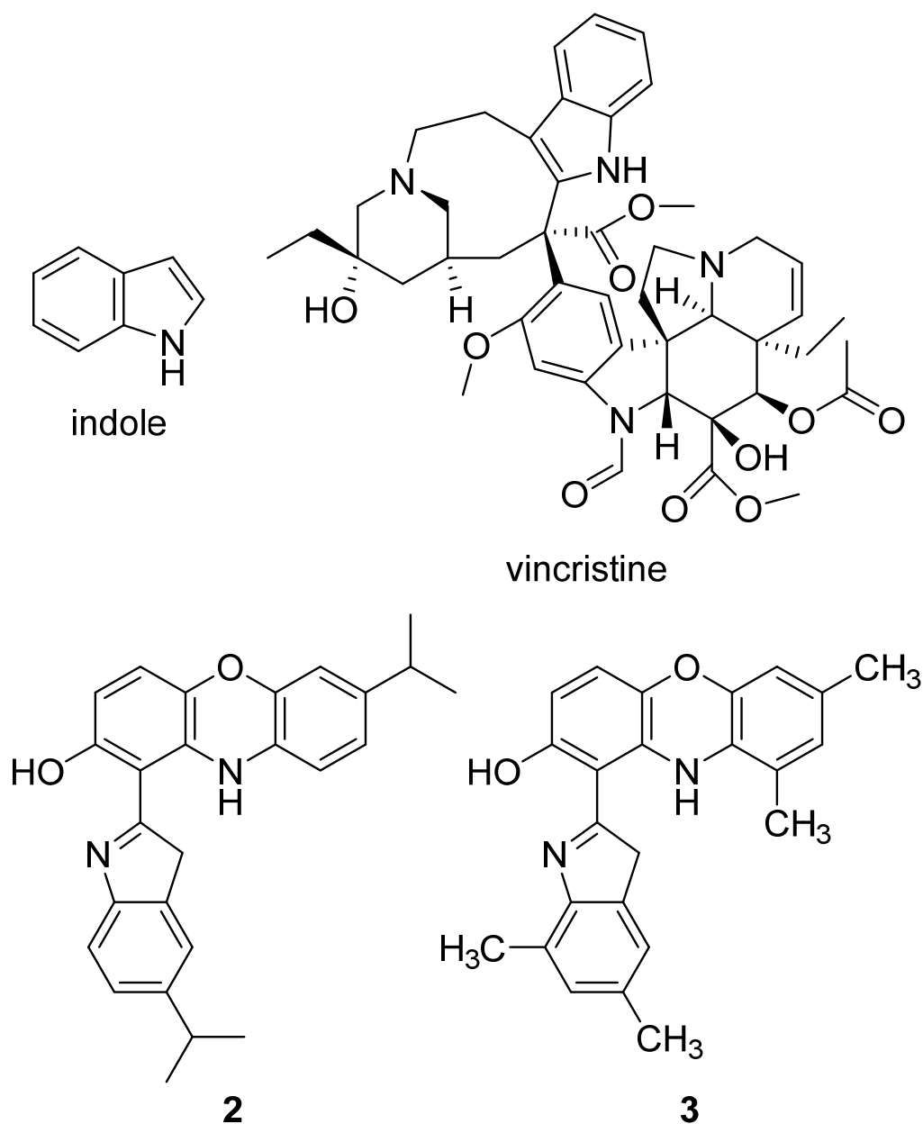
Figure 9. Structures of indole, the anticancer drug vincristine and the most active indole derivatives.
