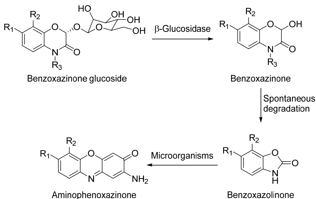
Scheme 1. General degradation process of benzoxazinones.
