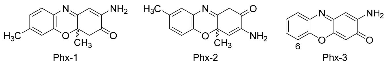
Figure 3. Most studied aminophenoxazinones: 2-amino-4,4 \alpha -dihydro-4 \alpha ,7-dimethyl-3H-phenoxazin-3-one (Phx-1), 3-amino-1,4 \alpha -dihydro-4 \alpha ,8-dimethyl-2H-phenoxazin-2-one (Phx-2) and 2-aminophenoxazine-3-one (Phx-3).
