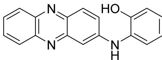
Figure 4. Structure of N -(2-hydroxyphenyl)-2-phenazamine (NHP).
