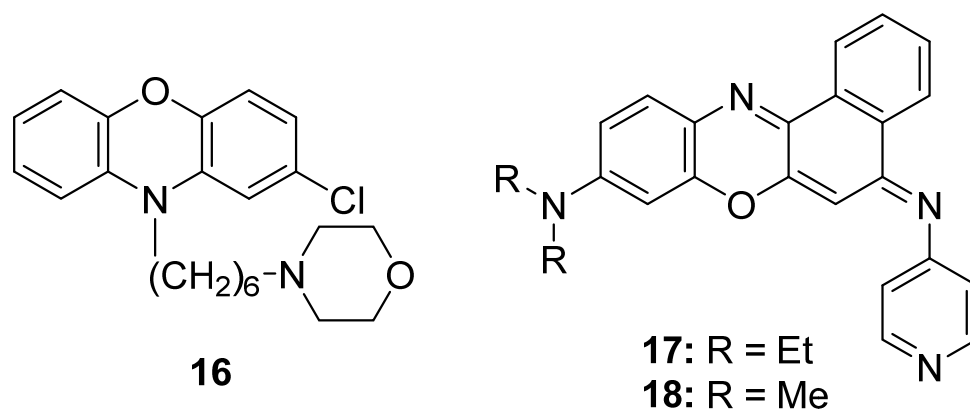
Figure 12. Phenoxazin derivatives with antibacterial (16) and antimalarial (17 and 18) activity.
