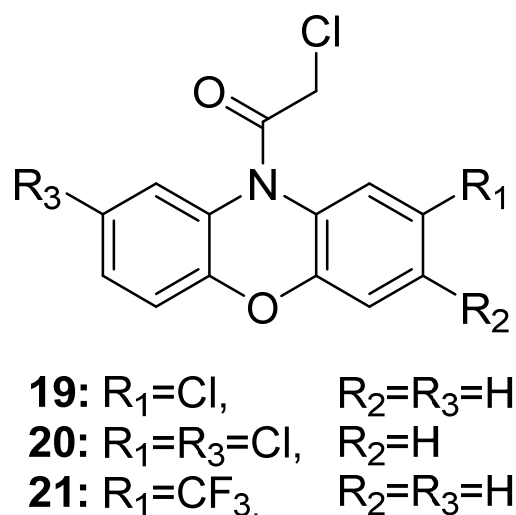
Figure 13. Compounds that have exhibited some interesting potential to treat L. major infections.
