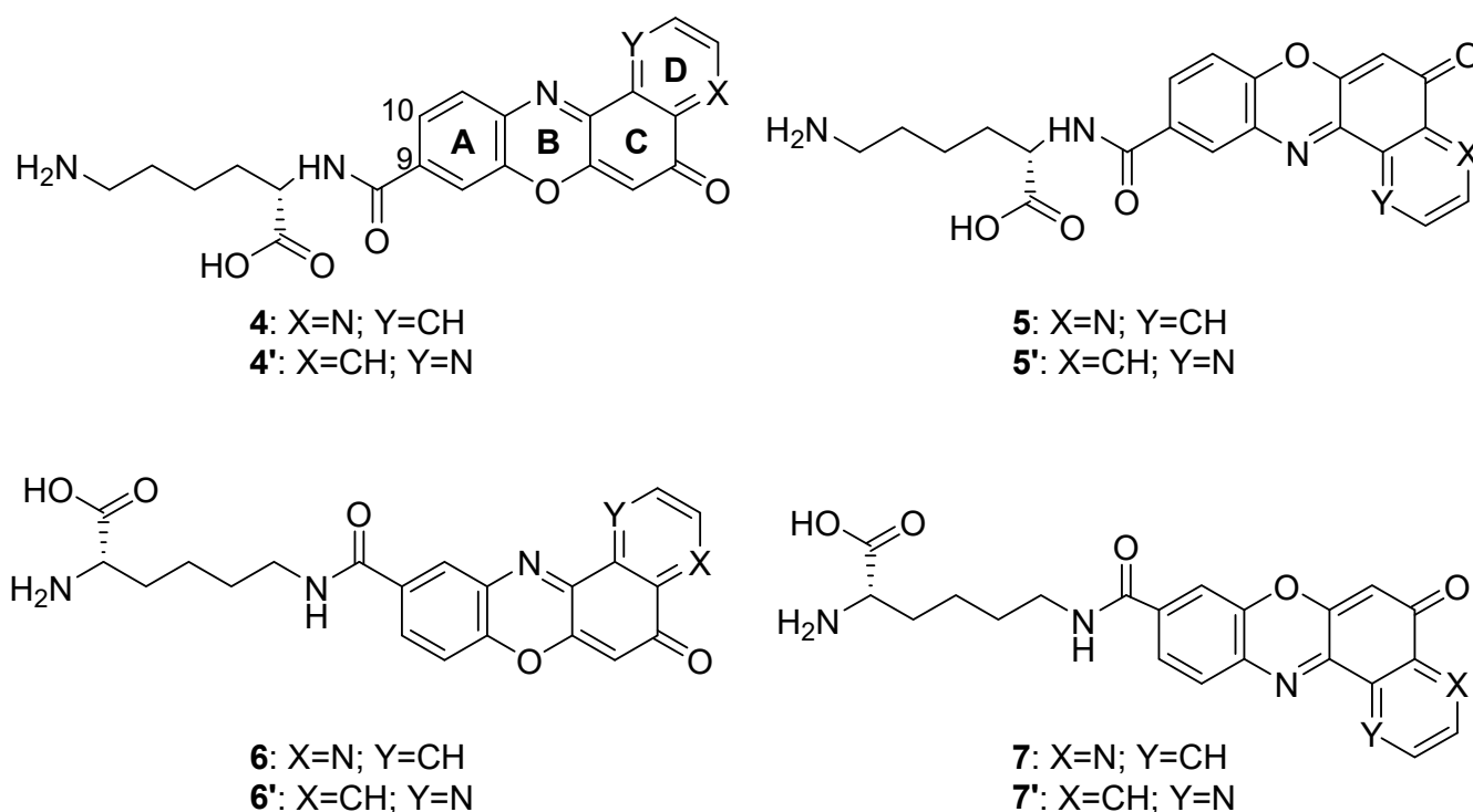
Figure 10. Structure of the pyridophenoxazinone derivatives conjugated to L-lysine.
