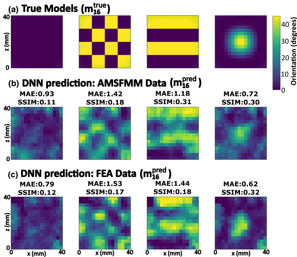
Fig. 6 a True material maps ( m_{16}^{true} ). The predicted models using the AMSFMM trained DNN tomography algorithm with b m_{16}^{pred} = DNN(T_m^{FMM}) and c m_{16}^{pred} = DNN(T_m^{FEA})
