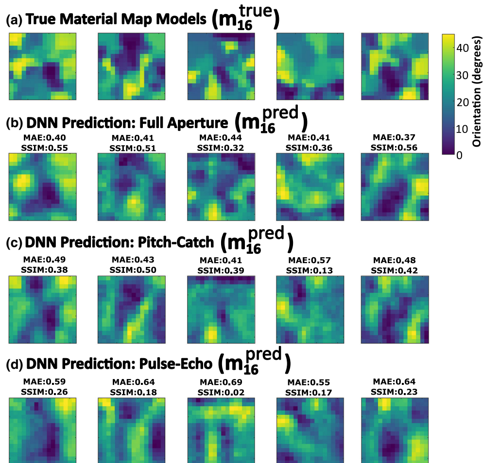
Fig. 4 a True material orientation maps \mathbf{m}_{16}^{\text{true}} from the test data set and corresponding predicted models \mathbf{m}_{16}^{\text{pred}} using the DNN tomography algorithm for b full aperture, c pitch-catch and d pulse-echo transducer array configurations. The associated mean absolute errors
