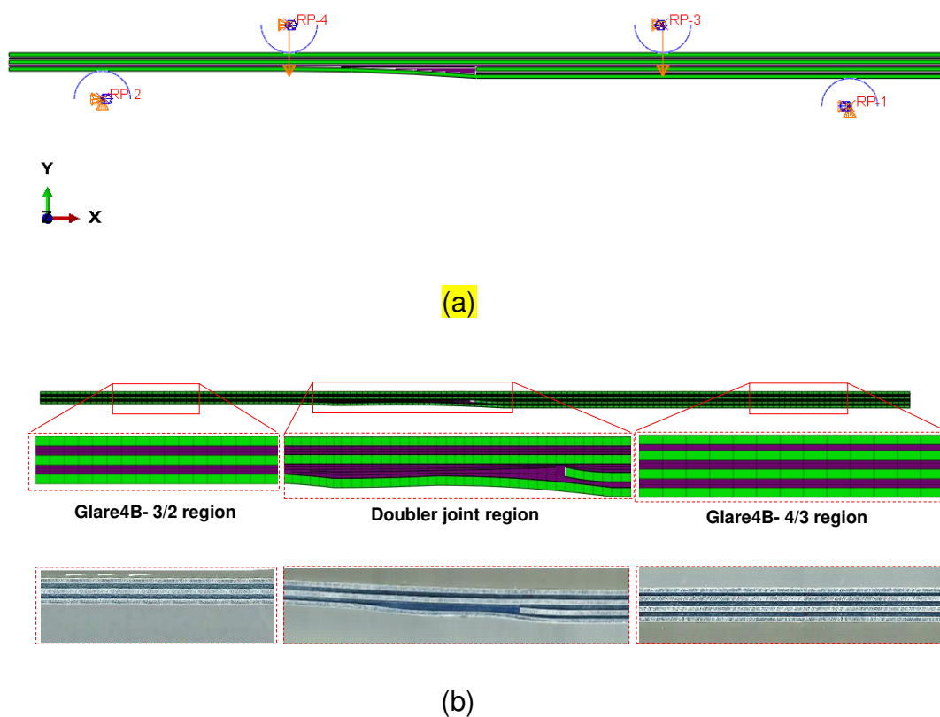
Figure 12: (a) Applied load and boundary conditions for the 4-point bending 2D FE model, (b) Finite element mesh of the doubler specimen (top) based on optical scans of real specimens (bottom) (images resized for clarity, not to scale).
