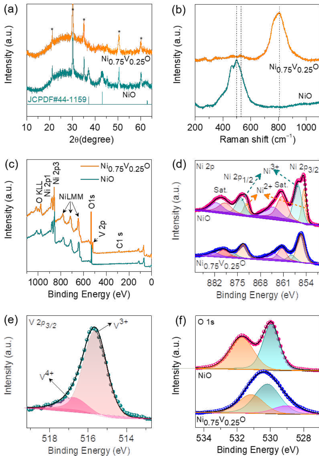
Figure 3. (a) X-ray diffraction patterns of NiO and Ni 0.75 V 0.25 O together with JCPDS standards (44-1159). (b) Raman spectra of NiO and Ni 0.75 V 0.25 O. XPS analysis of Ni 0.75 V 0.25 O: (c) survey spectra showing the presence of Ni, V, and O, (d) core level Ni 2p, (e) core level V 2p 3/2 , and (f) O 1s.
