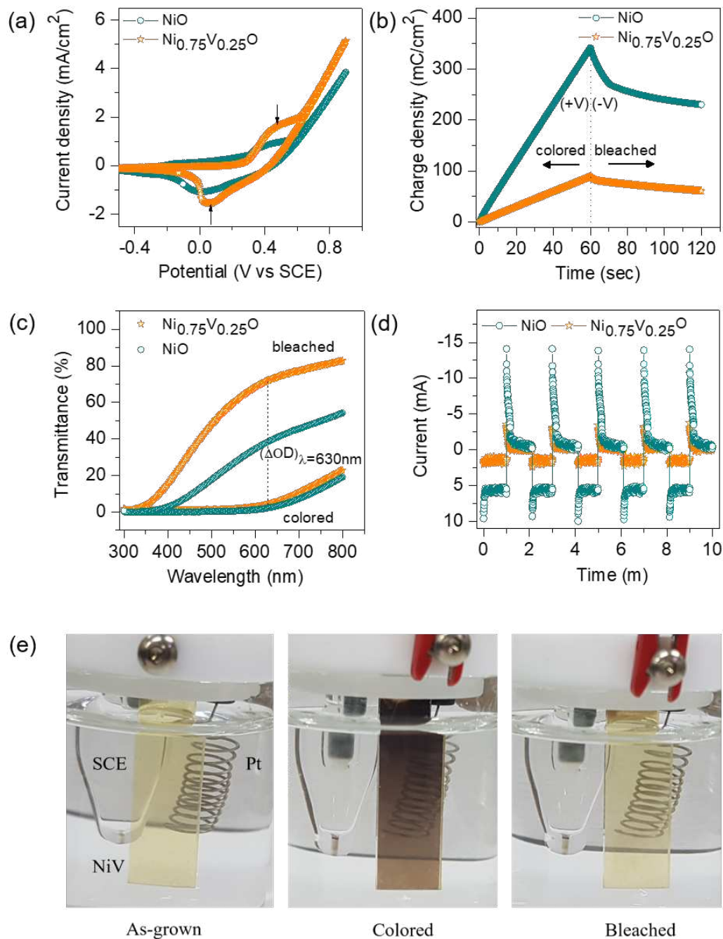
Figure 4. (a) Cyclic voltammogram of NiO and Ni 0.75 V 0.25 O recorded in a 2M KOH electrolyte at a scan rate of 5mV/s. (b) Chronocoulometry measurements for the colored film at ±0.6 V. (c) Optical transmittance spectra for NiO and Ni 0.75 V 0.25 O in a colored and bleached state. (d) Chronoamperometric curves for the Ni 0.75 V 0.25 O and NiO samples recorded with a potential step of ±1.2 V (vs. the SCE) for a fixed time of 60 s. (e) Images of Ni 0.75 V 0.25 O samples taken in a colored and bleached state.
