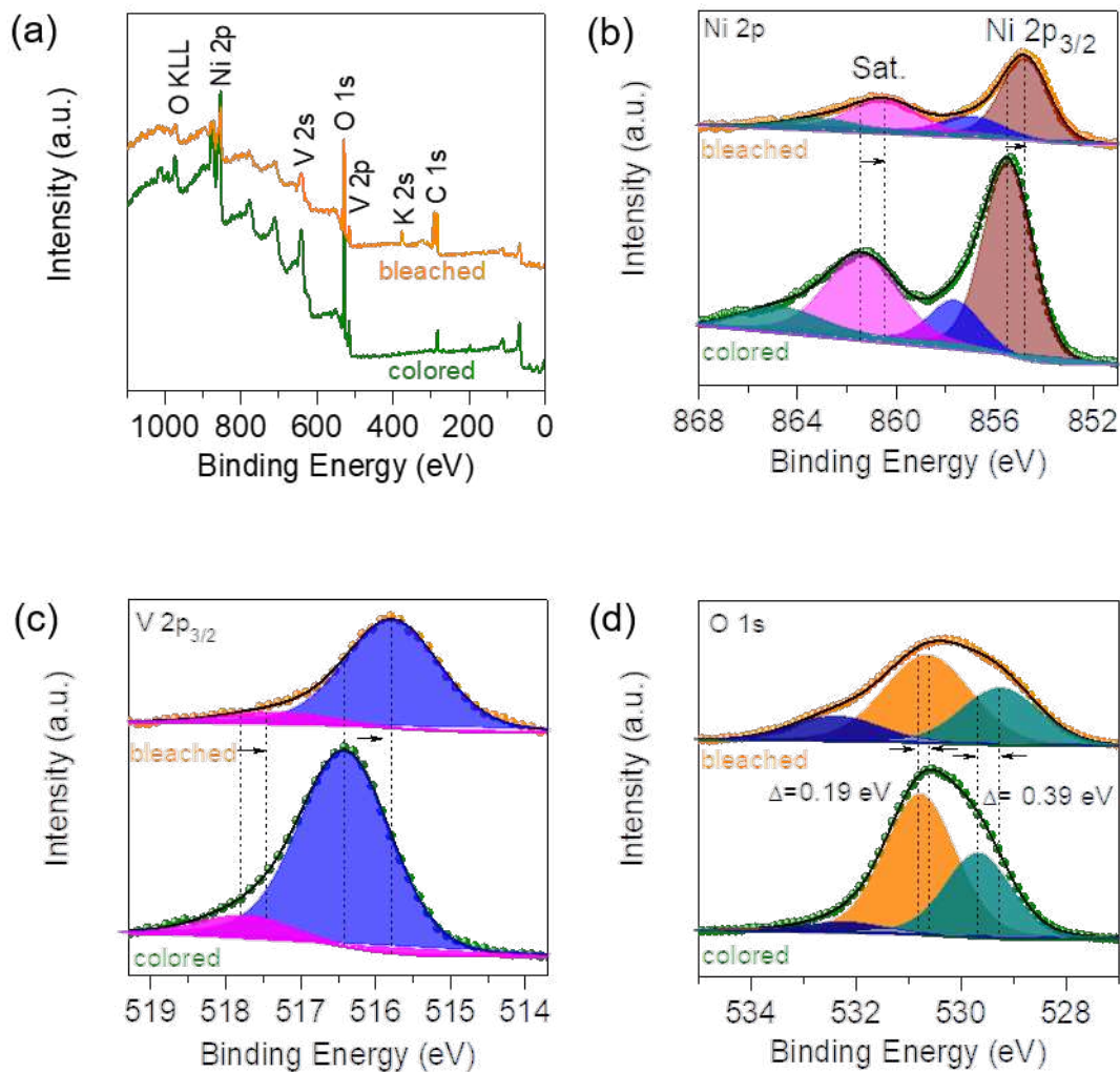
Figure 6. Ex-situ XPS analysis of \text{Ni}_{0.75}\text{V}_{0.25}\text{O} in a colored and bleached state: (a) survey spectra, (b) core-level Ni 2p_{3/2} revealing a shift towards higher energy after coloration, (c) core-level V 2p_{3/2} showing the oxidation of the electrode during the coloration process, and (d) core-level O 1s .
