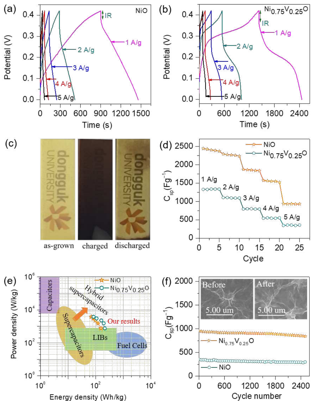
Figure 5. Galvanostatic charge–discharge (GCD) curves for (a) NiO and (b) Ni 0.75 V 0.25 O recorded at different current densities. (c) Images of Ni 0.75 V 0.25 O samples taken in a charged and discharged state. (d) Specific capacitance obtained from the GCD curves at various current densities. (e) calculated energy density and power density (Ragone plot). (f) Cycling stability test at a high current density of 5 Ag -1 for over 5000 charge–discharge cycles.
