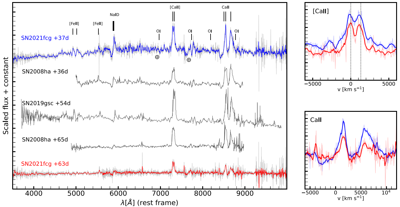
Figure 4. Left: late-time optical spectra of SN 2021fcg at +37 days (blue) and +63 days (red). Also plotted are similar phase spectra of SN 2008 ha and SN 2019gsc (gray; taken from Valenti et al. 2009; Tomasella et al. 2020). The spectra of SN 2021fcg closely resemble the spectra of the other low-luminosity SNIax. Right: zoom-in of the [Ca II] (top) and Ca II (bottom) emission lines. These are the strongest features in the spectra (37 days: blue, 63 days: red). In both spectra, the peak wavelengths of [Ca II] emission are blueshifted from the rest wavelengths (black dashed lines in the top panel) by \approx 100 \text{ km s}^{-1} . The optical spectra of SN 2021fcg are available as the data behind the figure.
