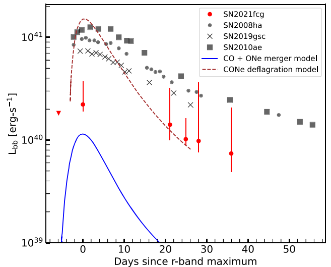
Figure 3. Bolometric luminosity evolution (derived from blackbody fitting) of SN 2021fcg compared with the blackbody luminosities of SNe 2008 ha, 2010ae, and 2019gsc (Srivastav et al. 2020). The peak luminosity of SN 2021fcg is smaller than the other low-luminosity SN Iax by a factor of \sim 3 . Also plotted are the theoretical bolometric luminosities of explosions from deflagration of a near- M_{\text{ch}} white dwarf (dashed brown line; Kromer et al. 2015) and the merger of a 1.1 M_{\odot} CO and a 1.2 M_{\odot} ONe white dwarf (solid blue line; Kashyap et al. 2018).
