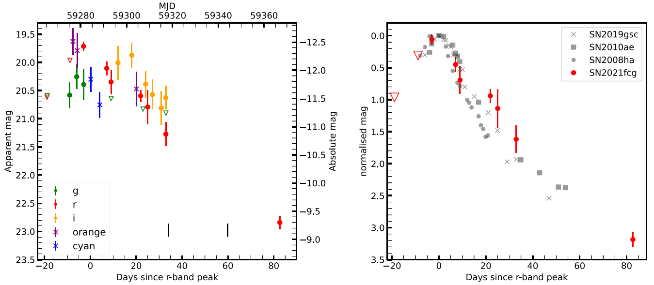
Figure 2. Left: g -, r -, i -, o -, and c -band lightcurve of SN 2021fcg. The epochs of our spectroscopic observations are marked with a black vertical line. Right: comparison of the r -band photometric evolution to other low-luminosity SN Iax (SNe 2008 ha, 2019gsc, and 2010ae). In the first 12 days post-maximum, the evolution of SN 2021fcg is similar to SNe 2010ae and 2019gsc, but slower than SN 2008 ha. After 12 days, the evolution of SN 2021fcg slows down, with a possible plateau between 12 and 22 days. This plateau is also seen in the i -band measurements (left panel). Data for the comparison objects are taken from Valenti et al. (2009), Stritzinger et al. (2015), and Srivastav et al. (2020), respectively. The lightcurve photometry of SN 2021fcg is available as the data behind the figure. (The data used to create this figure are available.)
