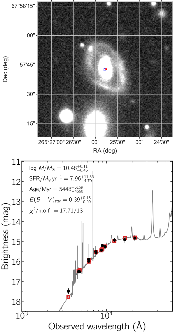
Figure 5. Host association and Properties: (Top panel) Location of nearby galaxies obtained from the Legacy Survey in g band from the NOAO data lab are shown along with the supernovae. The location of AT 2019lcj is indicated with a red cross, while SN 2020aewj is shown with a blue open square almost spatially coincident in the core of the host galaxy (Bottom Panel) The best fit model spectral energy distribution of the host galaxy of ZTF19aambfxc (photometric observations \bullet , model-predicted magnitudes \square ) from multi-band photometry. The solid line displays the best-fitting model of the SED. The fitting parameters are shown in the upper-left corner. The abbreviation n.o.f. stands for numbers of filters.
