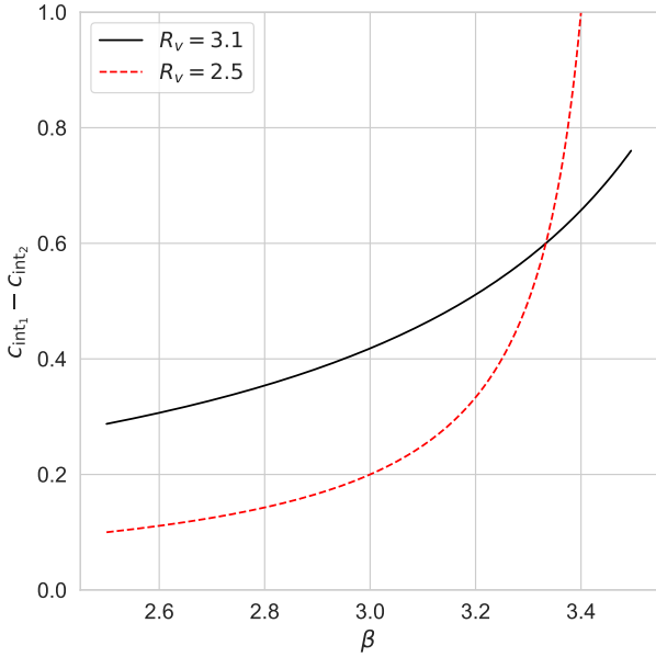
Figure B1. The differences in c_{int} in the model described in Brout & Scolnic (2021) for the pair of siblings described as a function of \beta (note that this is different from the SALT standardization model \beta constrained in Sec. 5 for two choices of R_V ).
