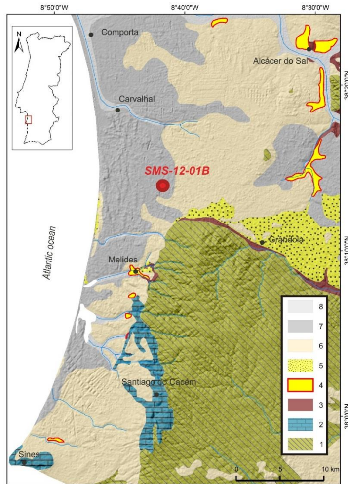
Figure 1. Simplified geological map of the study area showing the SMS-12-01B borehole location. 1, Paleozoic; 2, Mesozoic; 3, Paleogene (Vale do Guizo Formation); 4, late Serravalian-early Tortonian (Alcácer do Sal Formation); 5, Messinian (Esbarrondadoiro and Melides formations); 6, Zanclean-Gelasian (Ulme, Alvalade, Galé and Vale Figueira formations); 7, Holocene (aeolian and beach sands); 8, Holocene (alluvium). Cenozoic stratigraphy according to Antunes and Pais (1983), Antunes et al. (1991), Pimentel (1997), Pais et al. (2012), Ressurreição (2018), Cunha (2019). Adapted from published geological maps at 1:50 000 scale (Antunes and Pais, 1983; Antunes et al. , 1991; Inverno et al. , 1986; Dias et al. , 2011).
