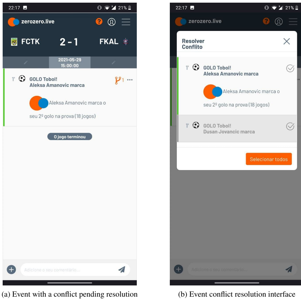
Figure 4.8: ZeroZero Live — Conflicts interface
