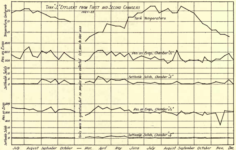
FIG. 20.—VARIATIONS IN EFFLUENT FROM CHAMBERS J1 AND J2 OF TANK J: FARM SEWAGE
