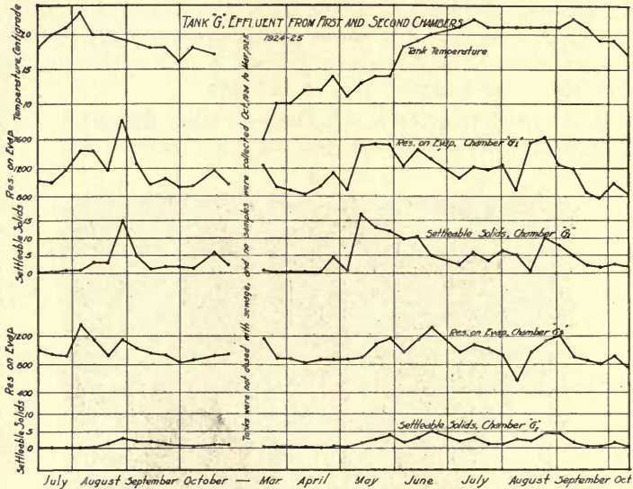
FIG. 19.—VARIATIONS IN EFFLUENT FROM CHAMBERS G1 AND G2 OF TANK G (FIG. 17): CITY SEWAGE
