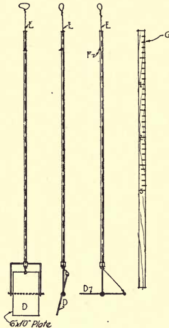
FIG. 8.—DEVICE FOR MEASURING THE THICKNESS OF SCUM
