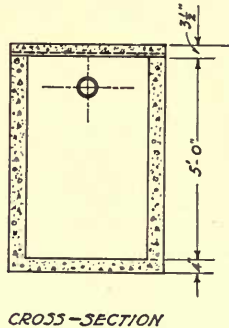
FIG. 24.—SUGGESTED DESIGN FOR A SINGLE-CHAMBER SEPTIC TANK
