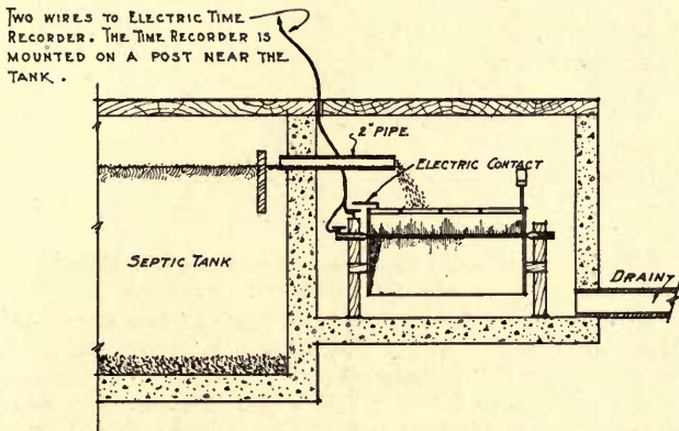
FIG. 2.—THE TIPPING-BUCKET METER SHOWN IN FIG. 1 INSTALLED IN A MANHOLE AT THE OUTLET END OF THE SEPTIC TANK
