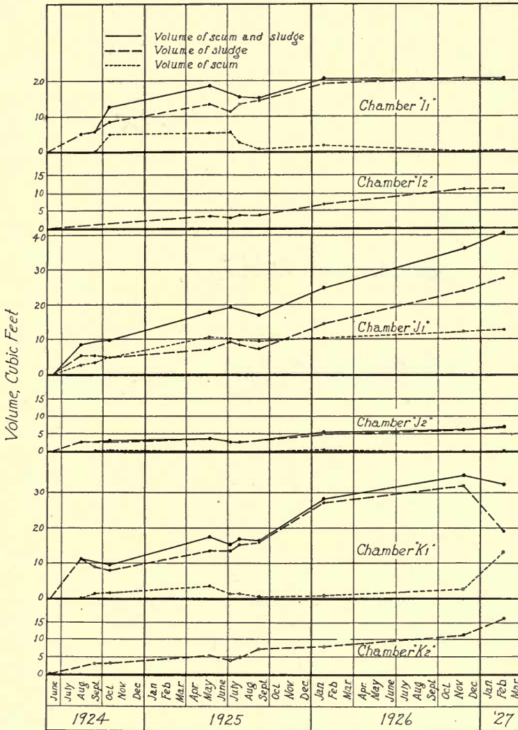
FIG. 22.—RATE OF SCUM AND SLUDGE ACCUMULATION WITH FARM SEWAGE
