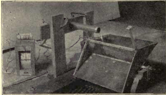
FIG. 1.—TIPPING-BUCKET METER FOR DETERMINING THE QUANTITY AND RATE OF SEWAGE FLOW FROM A FARM HOME
