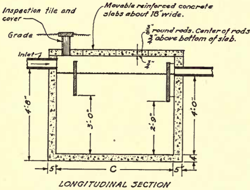
FIG. 24.—SUGGESTED DESIGN FOR A SINGLE-CHAMBER SEPTIC TANK
