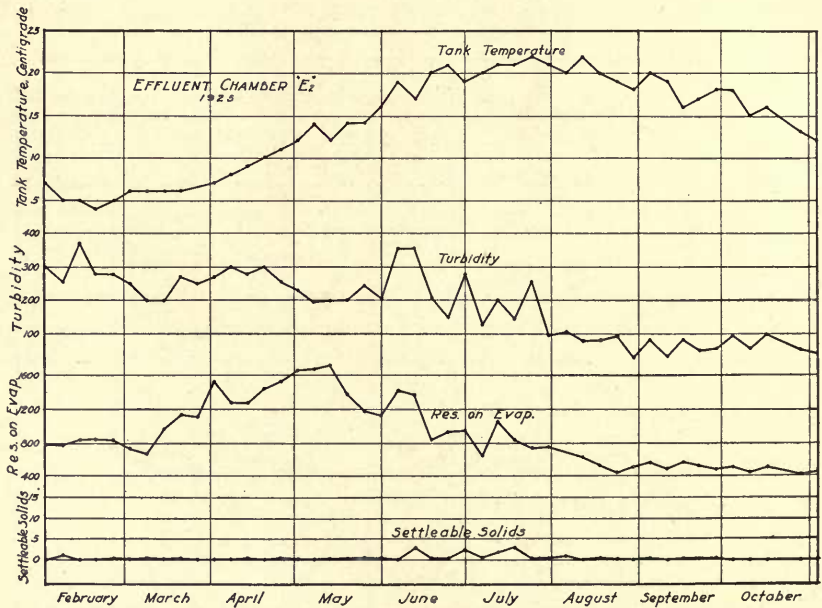
FIG. 16.—VARIATIONS IN EFFLUENT FROM CHAMBER E2, SECOND CHAMBER OF TANK E: FARM SEWAGE
