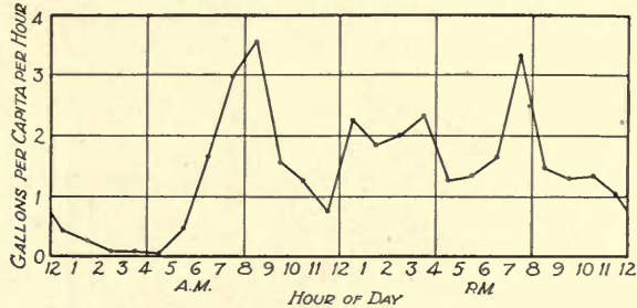
FIG. 3.—RATE OF SEWAGE FLOW FROM A FARM HOME OF THREE PEOPLE
