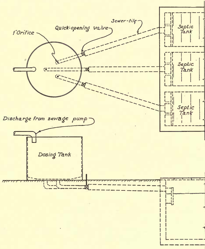
FIG. 5.—PLAN AND ELEVATION OF THE DOSING APPARATUS
