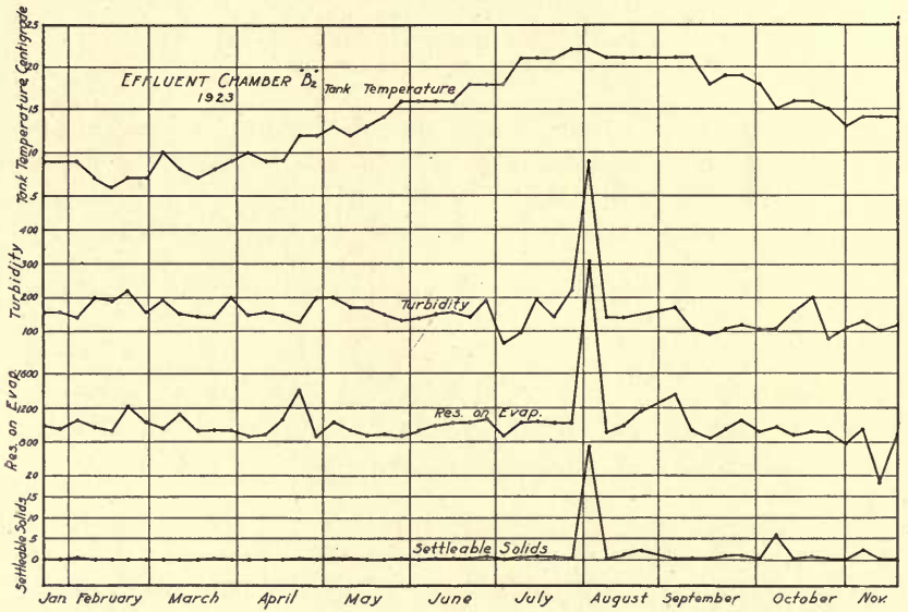
FIG. 12.—VARIATIONS IN EFFLUENT FROM CHAMBER B2, SECOND CHAMBER OF TANK B: CITY SEWAGE
