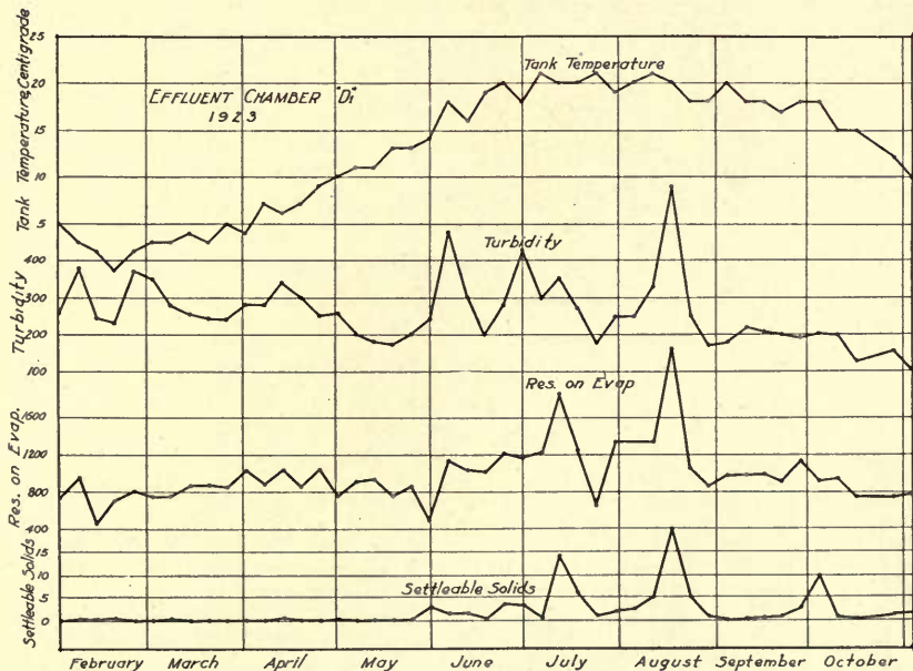
FIG. 14.—VARIATIONS IN EFFLUENT FROM CHAMBER D1, FIRST CHAMBER OF TANK D: FARM SEWAGE
