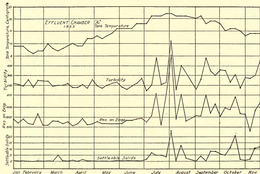
FIG. 10.—VARIATIONS IN EFFLUENT FROM CHAMBER A1, FIRST CHAMBER OF TANK A (FIG. 4): CITY SEWAGE
