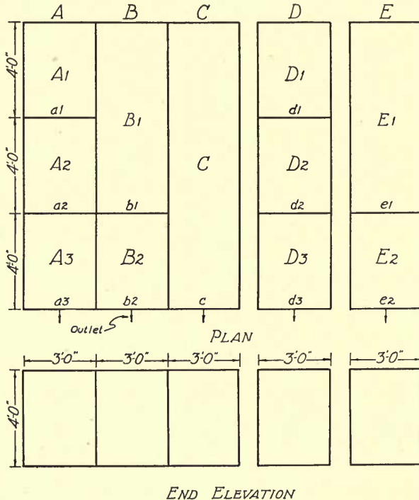
FIG. 4.—PLAN AND END ELEVATION OF EXPERIMENTAL SEPTIC TANKS USED IN STUDY II
