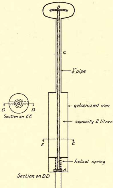
FIG. 7.—SEWAGE SAMPLING DEVICE
