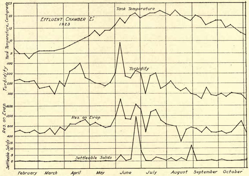
FIG. 15.—VARIATIONS IN EFFLUENT FROM CHAMBER E1, FIRST CHAMBER OF TANK E: FARM SEWAGE
