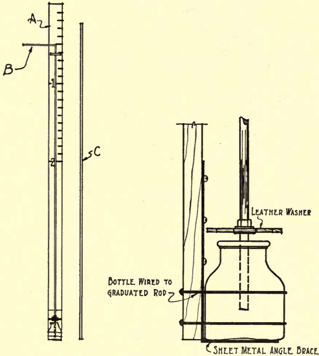
FIG. 9.—DEVICE FOR MEASURING THE DEPTH OF SLUDGE
