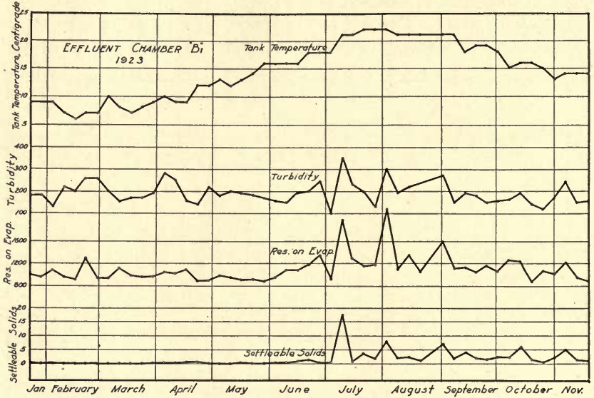
FIG. 11.—VARIATIONS IN EFFLUENT FROM CHAMBER B1, FIRST CHAMBER OF TANK B: CITY SEWAGE
