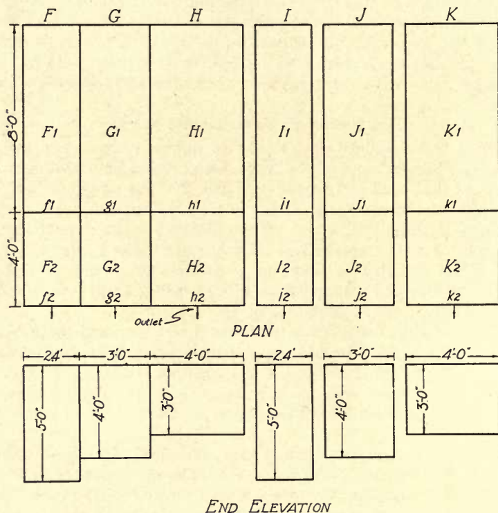
FIG. 17.—PLAN AND END ELEVATION OF EXPERIMENTAL SEPTIC TANKS USED IN STUDY OF DIFFERENTLY SHAPED CROSS-SECTIONS
