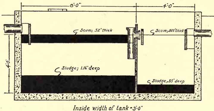
FIG. 23.—LONGITUDINAL SECTION OF TANK J
