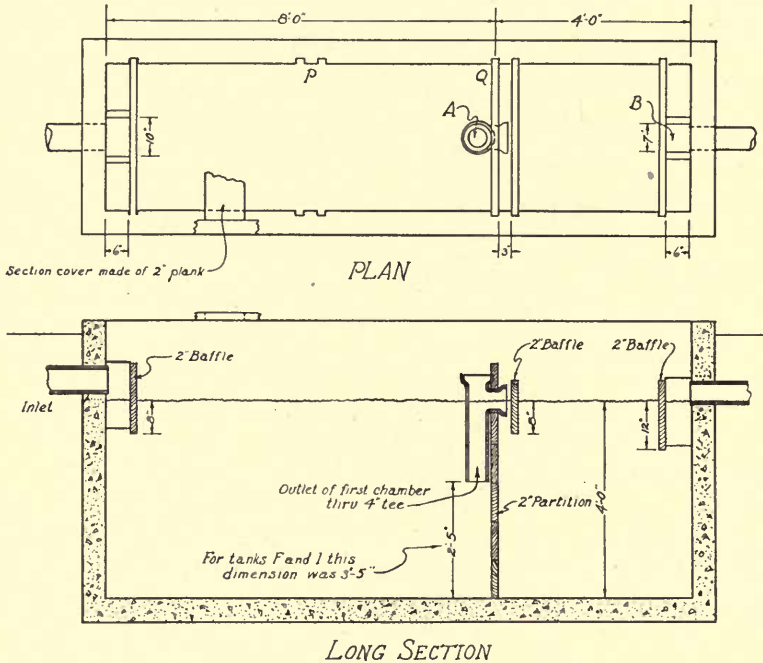
FIG. 6.—GENERAL DESIGN OF EXPERIMENTAL TANKS
