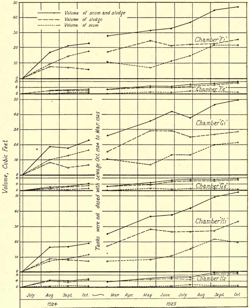
FIG. 21.—RATE OF SCUM AND SLUDGE ACCUMULATION WITH CITY SEWAGE
