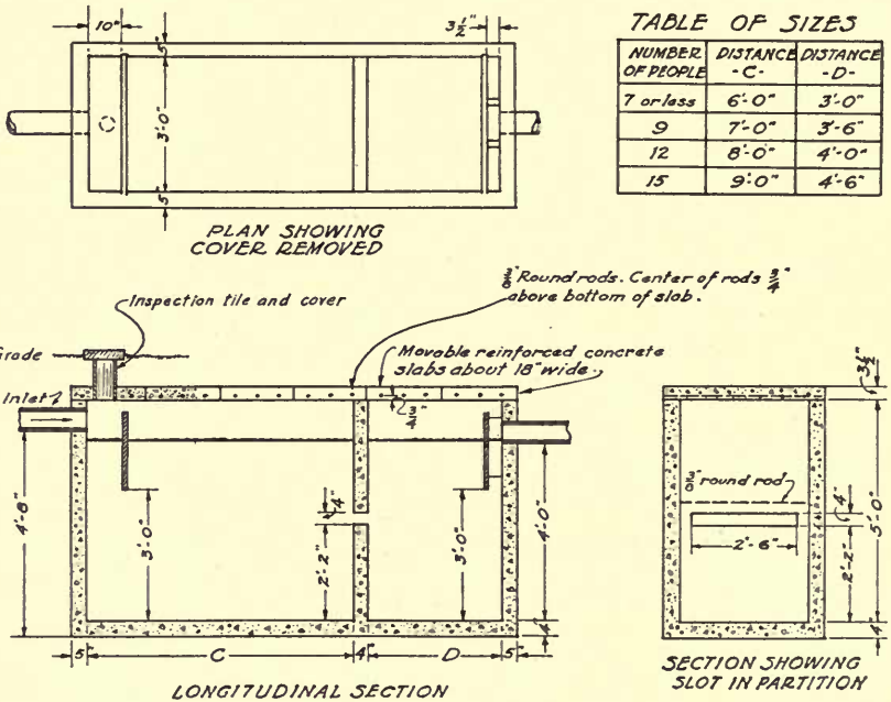
FIG. 25.—SUGGESTED DESIGN FOR A TWO-CHAMBER SEPTIC TANK
