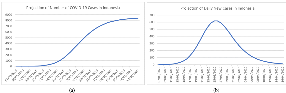
Figure 5: Predicting the number of COVID-19 case in Indonesia using parameter values for South Korea. (a) Prediction of the accumulated case, (b) Prediction of daily new case.
