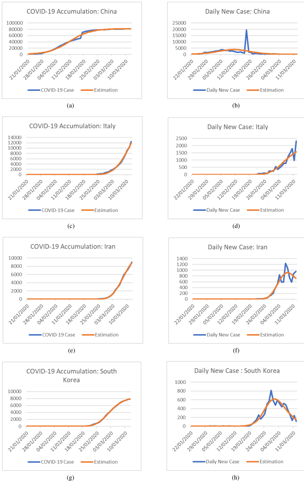
Figure 2: Data and prediction of number of people infected by nCOVid-19. Number of cases in each country is (a),(c),(e),(g) whereas (b),(d),(f),(h) is the number of daily cases.
