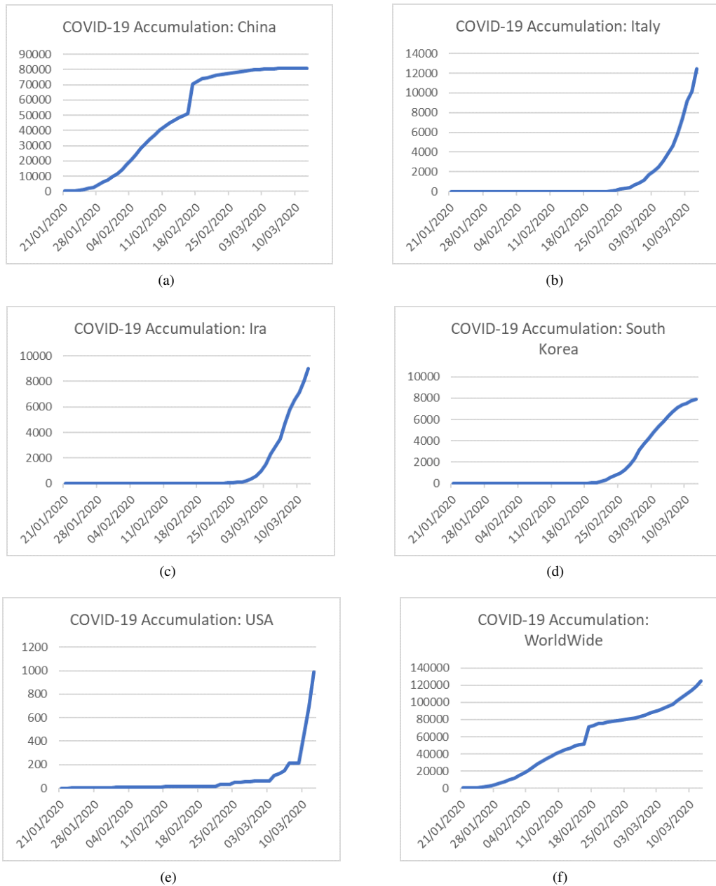
Figure 1: Number of infected from Januari 21 until March 13, 2020. (a) China, (b) Italy, (c) Iran, (d) South Korea, (e) USA, and (f) worldwide.
