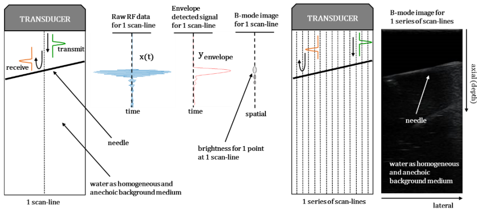
Figure 3 Needle image reconstruction in standard B-mode ultrasound image from raw RF data based on envelope detection.
