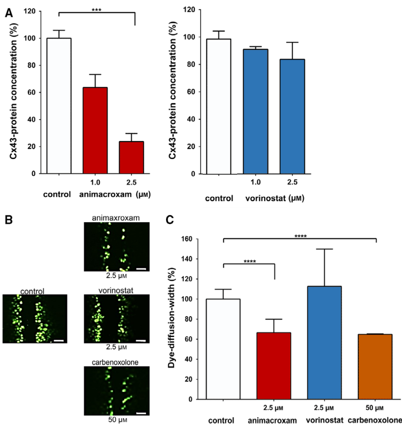
Fig. 6. Treatment-induced changes in Cx43 expression and endothelial cell–cell communication. (A) Protein expression of Cx43 was reduced after 24 h of incubation with animacroxam (1.0–2.5 μM) or—albeit to a lesser extent—with vorinostat (1.0–2.5 μM) when compared to control (100%). (B) Representative images of Lucifer Yellow dye diffusion in endothelial EA.hy926 cells after incubation with animacroxam or vorinostat; scale bar = 100 μm. (C) Lucifer Yellow dye diffusion, indicating intercellular gap-junctional cell–cell coupling, was diminished after 24 h of incubation with animacroxam (2.5 μM). This effect was absent after incubation with vorinostat (2.5 μM). The established Cx43 inhibitor Cbx (50 μM) served as a positive control. Results are shown as means ± SEM of at least n = 3 independent experiments. *** P -values of \leq 0.0005 , **** P -values of \leq 0.0001 ; one-way ANOVA post hoc Tukey's test.
