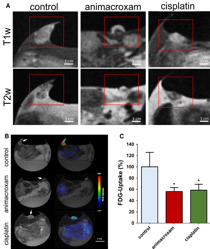
Fig. 2. Animacroxam induces ‘cap formation’ and suppresses glucose uptake in inoculated TGCT plaques. (A) T1w and T2w images of control-, animacroxam-, and cisplatin-treated tumor plaques. Animacroxam-treated tumors show a distinct viable tumor core (dark in T1w-/bright in T2w images) and a necrotic cap (bright in T1w-/dark in T2w images). (B) T1w and corresponding PET-MR images of 18F-FDG uptake in tumor plaques treated with NaCl, animacroxam, or cisplatin. (C) Animacroxam (5.0 \mu\text{M} )- and cisplatin (2.5 \mu\text{M} )-treated tumor plaques showed a reduced uptake of 18F-FDG. Results are shown as means \pm SEM of at least n = 3 independent experiments. Scale bar = 1 cm. * P -values of \leq 0.05 , unpaired t -test.
