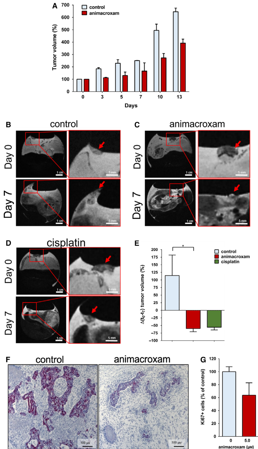
Fig. 1. Antineoplastic effects of animacroxam and cisplatin in vivo . (A) Relative tumor volume of TGCT xenografts grown in athymic nude mice after the treatment with 0.9% NaCl or animacroxam (daily dose of 60 mg·kg -1 body weight on four consecutive days, intraperitoneal). Results are shown as mean ± SEM of n = 2 mice in each group. (B–D) T2w MR images of tumor-bearing CAMs of fertilized chicken eggs taken before and after 7 days of a single intravenous injection with 0.9% NaCl (B), 5.0 μM animacroxam (C), or 2.5 μM cisplatin (D); scale bar = 1 cm (left side) or 0.5 cm (right side). (E) Mean changes in tumor volume of n = 3 CAM experiments. (F) IHC staining of Ki67 (red–violet) revealed a pronounced reduction of proliferation in animacroxam-treated tumors as compared to untreated controls; scale bar = 100 μm. (G) Quantification of Ki67-positive cells as a marker for proliferation in tumors excised out of the CAM after incubation with animacroxam (5.0 μM). Results are shown as mean ± SEM of n = 4 independent preparations. * P -values of ≤ 0.05, unpaired t -test.
