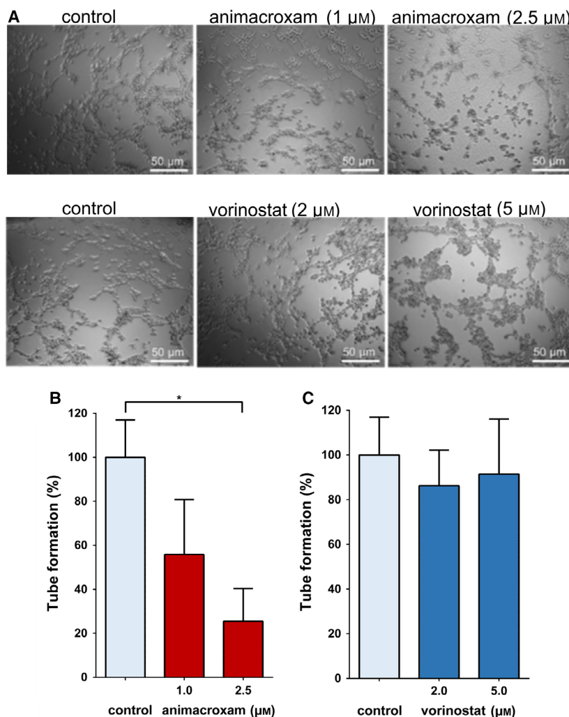
Fig. 5. Capillary-like tube formation is reduced after incubation with animacroxam. (A) Representative images of untreated and animacroxam (1.0–2.5 μM) EA.hy926 cells show a strong and dose-dependent reduction of tube-like structures after animacroxam treatment when compared to the control (100%). EA.hy926 cell-treated vorinostat (2.0–5.0 μM) displayed only minor reductions of tube-like structures when compared to the control (100%); scale bar = 50 μm. (B) Quantification of the tube formation compared to the untreated control after incubation with animacroxam (1.0–2.5 μM). (C) Quantification of the tube formation compared to the untreated control after incubation with vorinostat (2.0–5.0 μM). Results are shown as means ± SEM of n = 3 independent experiments. * P -values of \leq 0.05 ; one-way ANOVA post hoc Tukey's test.
