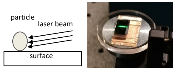
Figure 1: left) Laser surface cleaning at grazing incidence schematics; right) Laser surface cleaning of silicon wafer in action.
