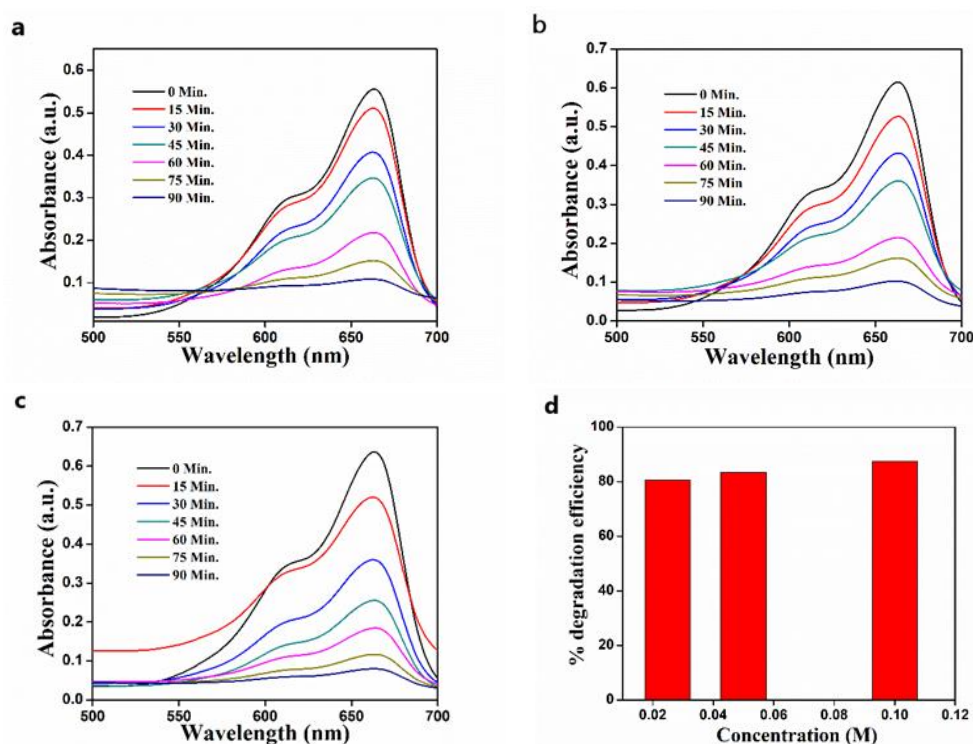
Figure 12. The photocatalytic degradation of MB after treatment with ZnO synthesized from (a) 0.025 M Zn(NO 3 ) 2 ; (b) 0.05 M Zn(NO 3 ) 2 ; (c) 0.1 M Zn(NO 3 ) 2 ; (d) the effect of Zn(NO 3 ) 2 ·6H 2 O concentration on photodegradation of MB.
