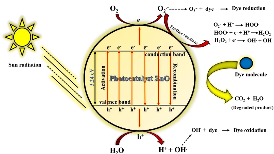
Figure 8. Schematic diagram of photocatalysis mechanism of ZnO NPs.
