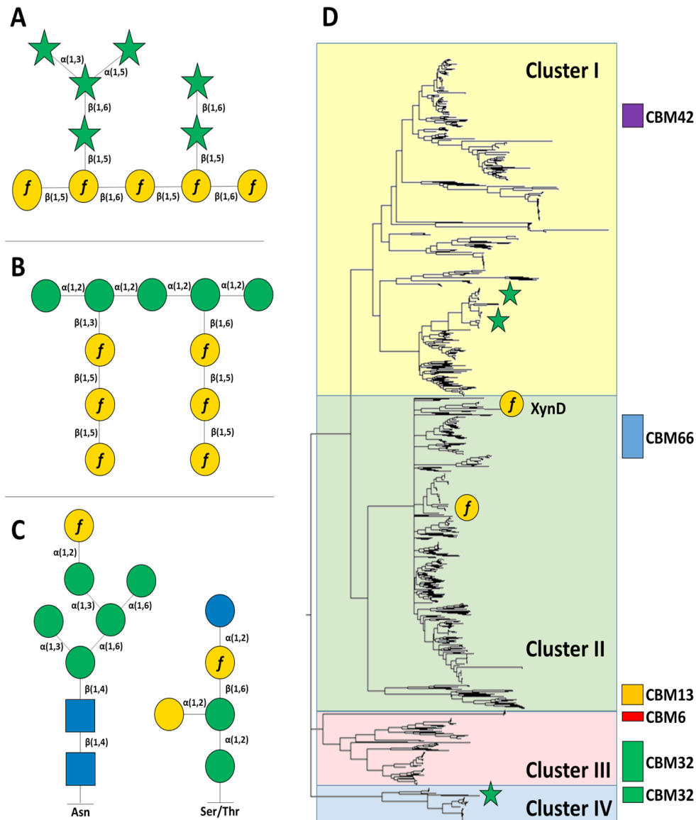
Figure 1: The presence of Galf throughout the fungal and bacterial kingdoms is not uniform and contains a variety of structures of both Galf backbones and Galf side chains, for example. a Structure of M. tuberculosis arabinogalactan fragment, b A. fumigatus galactomannan fragment, c N- and O-linked glycans. d Phylogenetic tree of GH43_34 family proteins with distinct clades visualised. Known activities are demonstrated as follows: \beta -galactofuranosidase (yellow circle), \alpha -arabinofuranosidase (green star).
