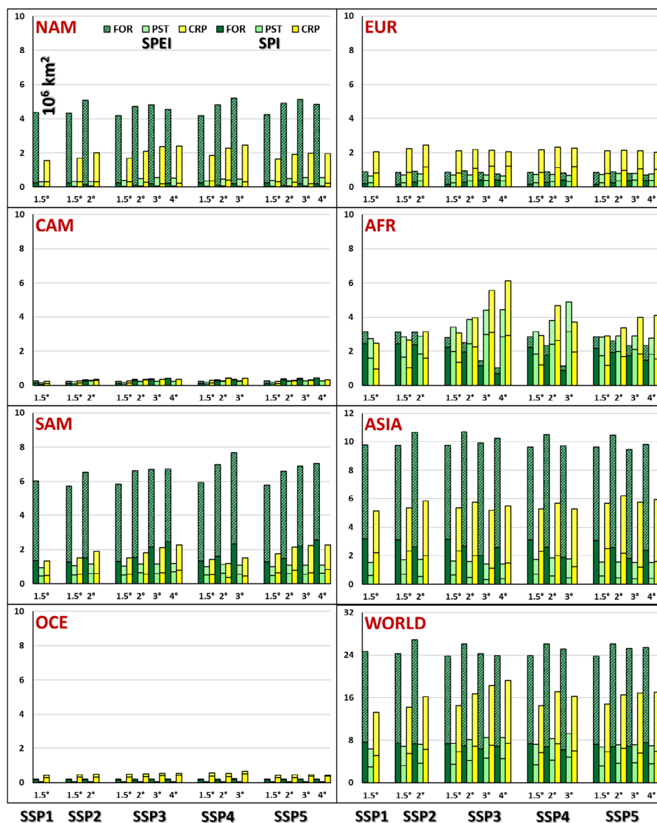
FIGURE 7 Land-use forests, pastures, and croplands, expressed in million km 2 , significantly exposed to at least one unprecedented event for a combination of SSPs and GWLs. Values are shown for both SPI (full columns) and SPEI (dashed) [Colour figure can be viewed at wileyonlinelibrary.com ]
