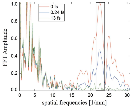
Figure 12 Normalized FFT for real mirrors. The black vertical line marks the area that is integrated in order to calculate the correlation function.
