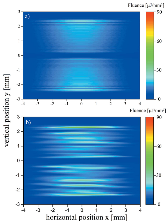
Figure 6 The separated transverse profile of both partial beams on an imaging detector at z = 972 m containing (a) ideally flat and (b) real mirrors. The FWHM in horizontal direction is D_{\text{FWHM}} = 5.2 mm.
