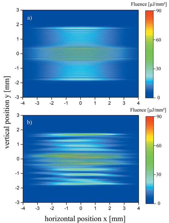
Figure 11 The transverse profile on an imaging detector at z = 972 m for (a) ideal and (b) real mirrors and an overlap of \Delta y_d = 0.75 mm (20% of the beam profile).
