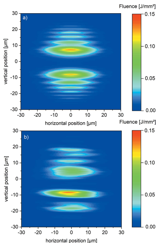
Figure 7 The separated transverse profiles on an imaging detector located at the focal spot at z = 972 m containing (a) ideal flat and (b) real mirrors for one possible lens configuration in the HED tunnel.
