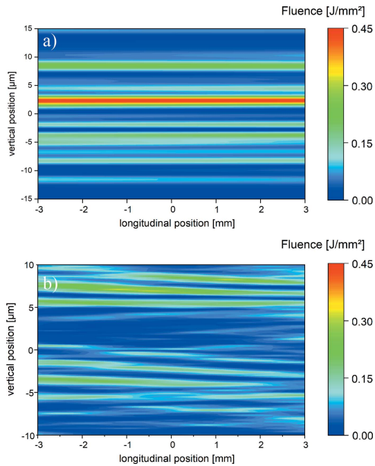
Figure 10 Vertical cuts for \tau = 0 fs at x = 0 for \Delta z = \pm 3 mm around the focal spot at z = 972 m using real mirrors including two offset mirrors for one possible lens configuration in the HED tunnel. In Fig. 10(a) only the intense parts are overlapped and Fig. 10(b) displays a nominally full overlap.
