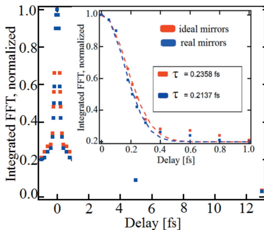
Figure 13 The simulated measurement of the temporal coherence properties of the SASE pulses for the ideal case (red labels) and the real case (blue labels). A Gaussian function with a constant background of V = 0.2 fit to values for delays between \tau = 0 fs and \tau = 1 fs (inset) yields a coherence time of \tau_c = 0.235 fs (HWHM) for the ideal case and \tau_c = 0.213 fs (HWHM) for the real case.
