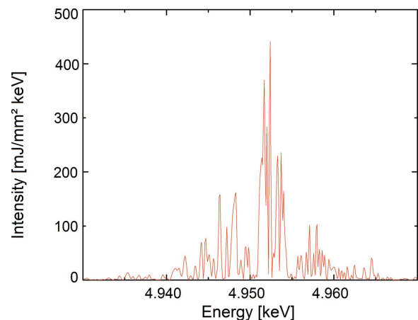
Figure 3 The spectrum of the FEL pulse that was used for the wavefront propagation simulation.
