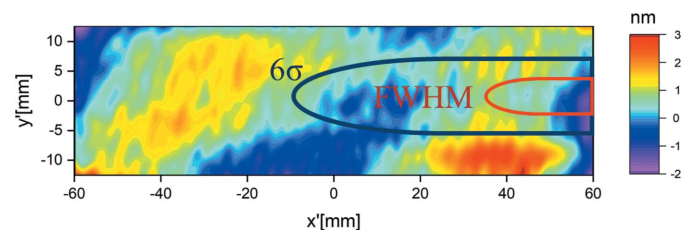
Figure 2 Topography of the beam splitter. The 6\sigma (blue) and the FWHM (red) footprint at h\nu = 5 \text{ keV} are indicated. Within the blue and red labeled area the maximum height deviations amounts to \Delta h = 3 \text{ nm} .
