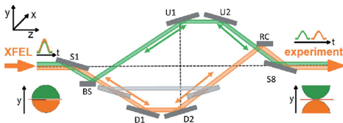
Figure 1 Schematic drawing of the optical layout of the hard X-ray split-and-delay unit (Roling et al. , 2012).
