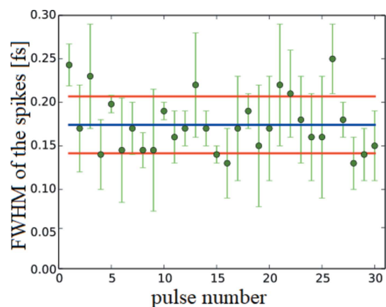
Figure 14 Averaged FWHM values of the spikes for different SASE pulses (green) are depicted. In addition, the ensemble averaged value for all SASE pulses (blue) is shown which is \bar{\tau}_{c,\text{pulses}} = 0.174 fs. The red lines mark the standard deviation of \bar{\tau}_{c,\text{pulses}} which is \Delta\tau = 0.034 fs. This figure thus exemplifies the shot-to-shot fluctuation of the theoretically calculated SASE pulses (Saldin et al. , 1999).
