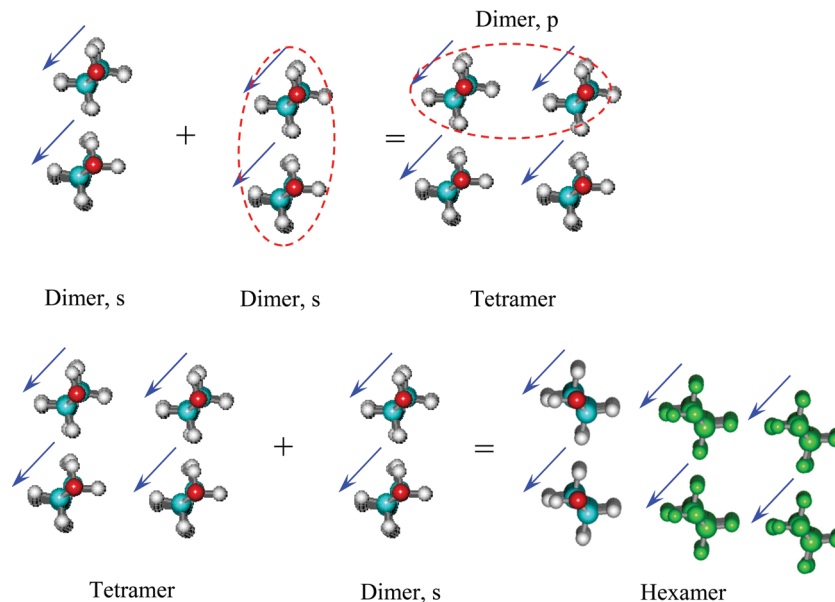
Fig. 2 Scheme of the formation of oblique films of aliphatic alcohols.
