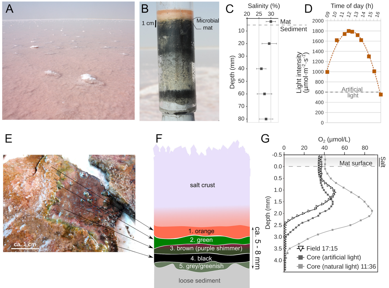
FIG 1 Overview of the sabkha near Shannah, Oman, and the salt covered microbial mats in February 2018. (A) Image of the sampling site in the salt-crust-covered tidal flat. (B) A core including sediment, microbial mat, salt crust, and salt-saturated water. (C) Depth profile of porewater salinity. Squares indicate average values from three cores, and error bars indicate standard deviation. (D) Light intensity measured over the course of a day with a PAR sensor. (E) A piece of microbial mat cleaned from the salt and with layers partially scraped off. (F) Scheme of mat layers based on observations of color and texture. (G) Representative microsensor profiles of \text{O}_2 concentrations in the mats measured during the sampling campaign (at 30% salinity). Profiles were measured in the field and in sampled cores with artificial and natural illumination. Sunrise and sunset times are indicated to consider differences in light intensity.
