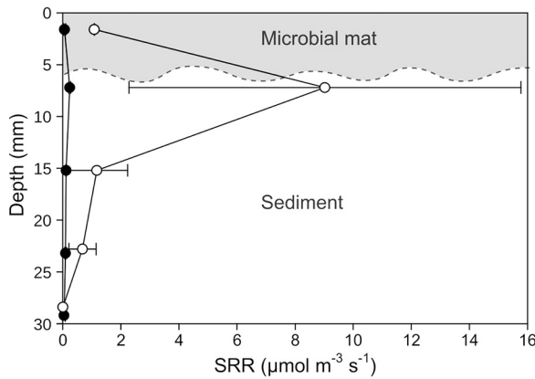
FIG 4 Sulfate reduction rates (SRR), determined by the 35 S method, in mats covered by a salt crust (black circles) and in mats after a simulated flood event (white circles). The dashed line indicates an approximate delineation between mat and sediment. Considering the slightly varying mat thickness, the peak of sulfate reduction might lie in the lowest mat layer or in the sediment directly underneath the mat.
