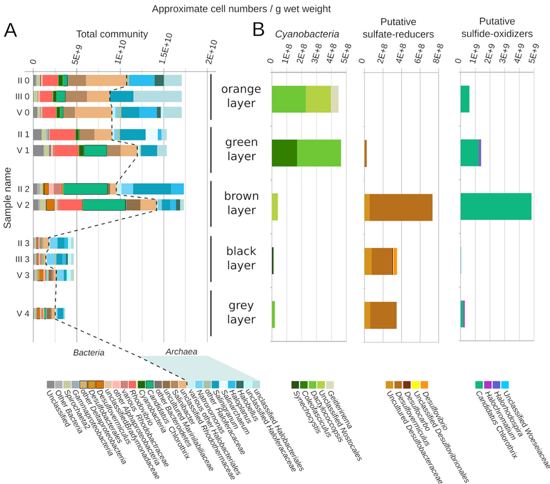
FIG 7 Microbial community composition as determined by 16S rRNA gene amplicon sequencing. The relative amplicon sequence abundances were multiplied by total cell counts per gram sediment obtained via fluorescence microscopy (see Fig. S7 in the supplemental material) as follows: (\text{Cell number/g sediment})_{\text{TAXON}} = (\text{Relative sequence abundance})_{\text{TAXON}} \times (\text{Total cell numbers/g sediment}) . (A) The composition of the total microbial community shown for two to three replicates per layer (exception layer 4 to 5 mm). In the sample name, the roman number indicates the mat patch replicate and the arabic number indicated the layer from "0" being the surface orange layer to "4" being the bottom gray layer. (B) Estimated cell numbers of photoautotrophs ( Cyanobacteria ), sulfate-reducing bacteria (all Deltaproteobacteria ), and sulfur-oxidizing bacteria in each layer. Full data on relative sequence abundances is provided in File S1 in the supplemental material.
